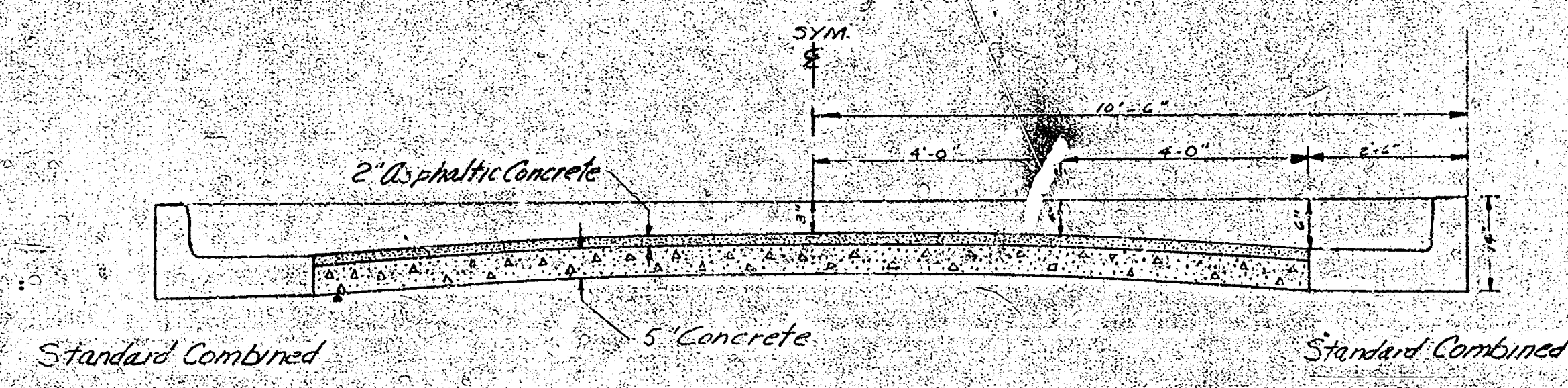
TYPICAL SECTION No Scale
