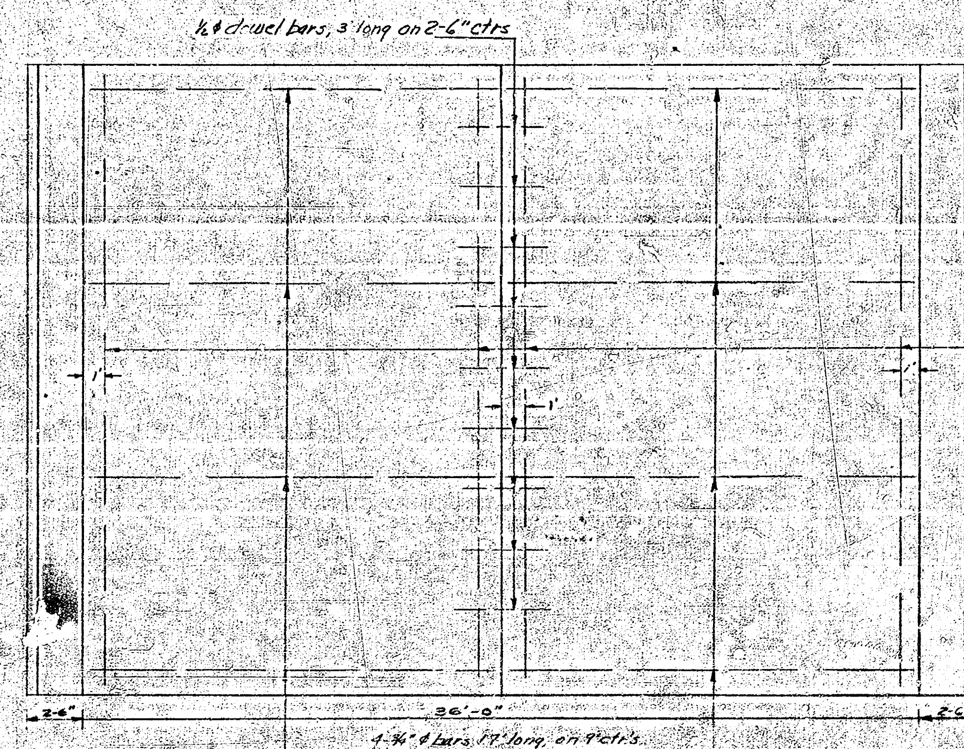
STEEL PATTERN Scale 4"=1'
