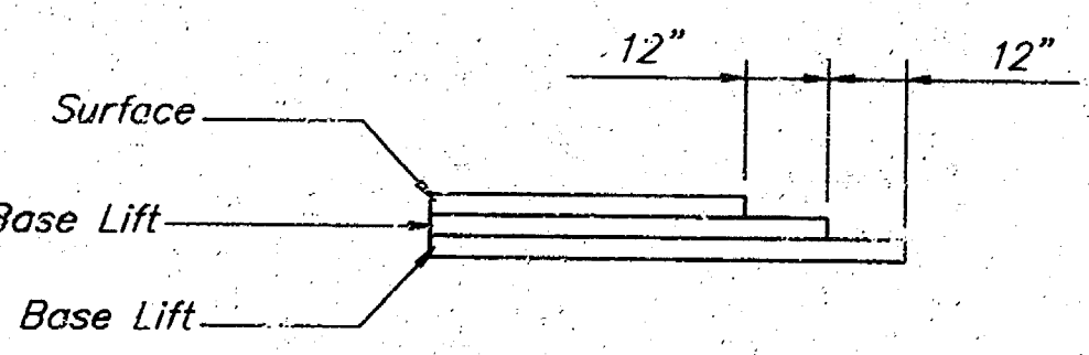
TRANSVERSE CONSTRUCTION JOINTS
