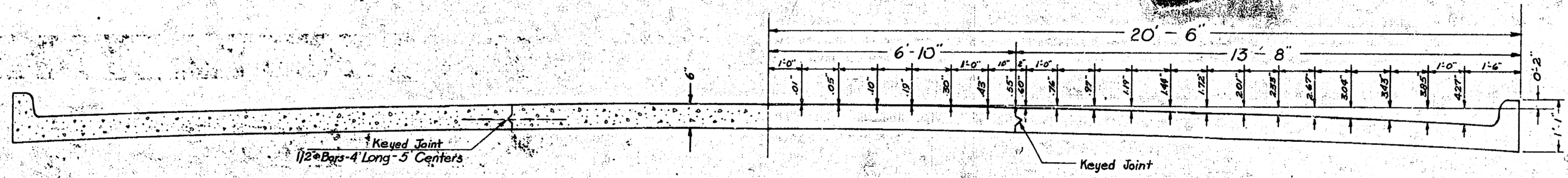
TYPICAL SECTION NO SCALE
