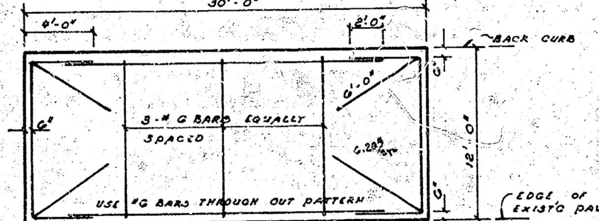
TYPICAL STEEL PATTERN
