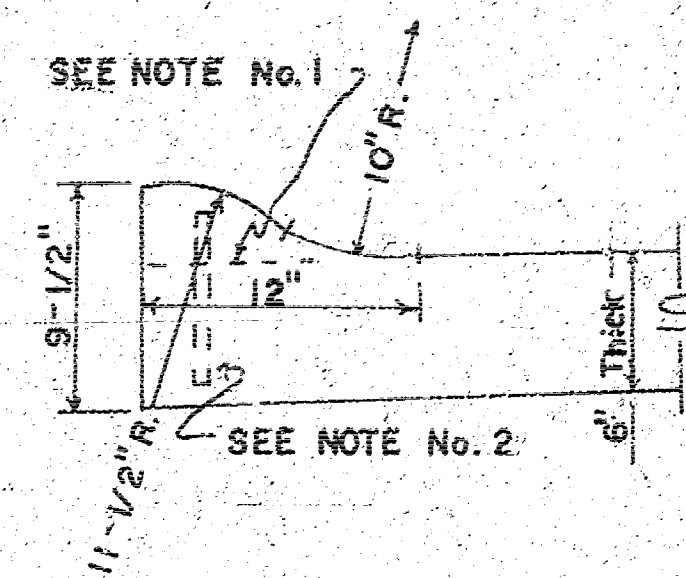
ROLL -TYPE
