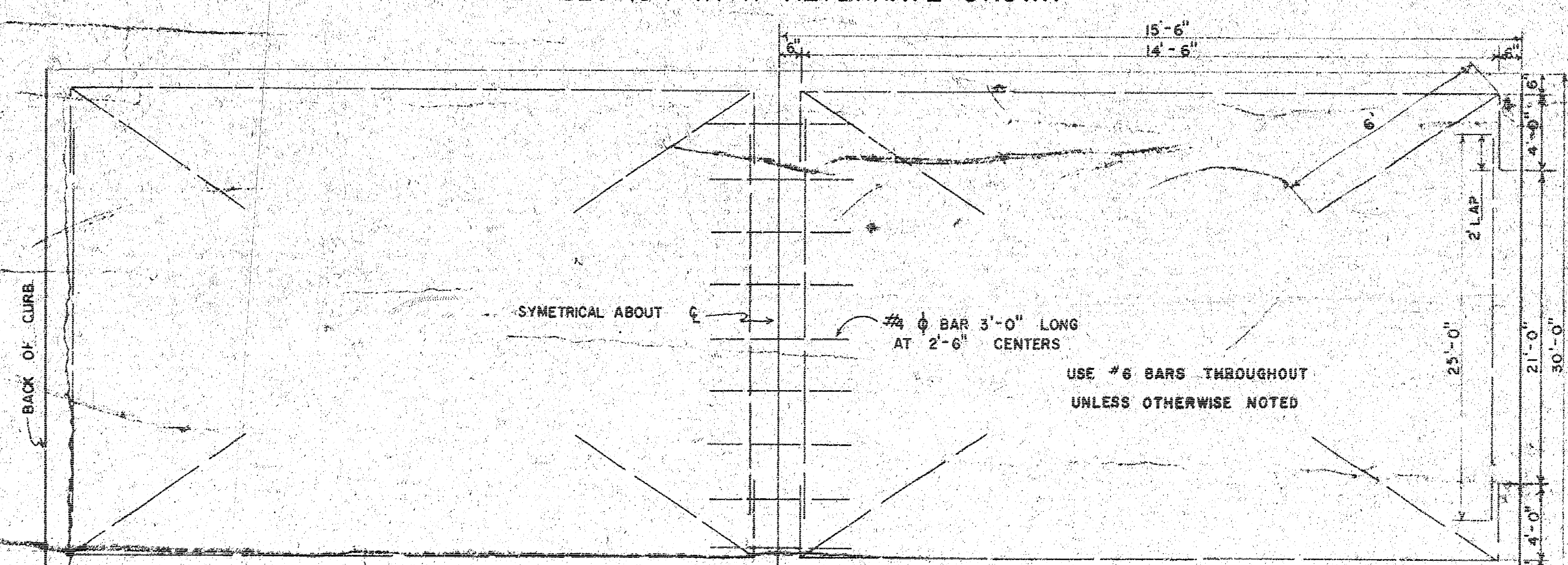
STEEL PATTERN
