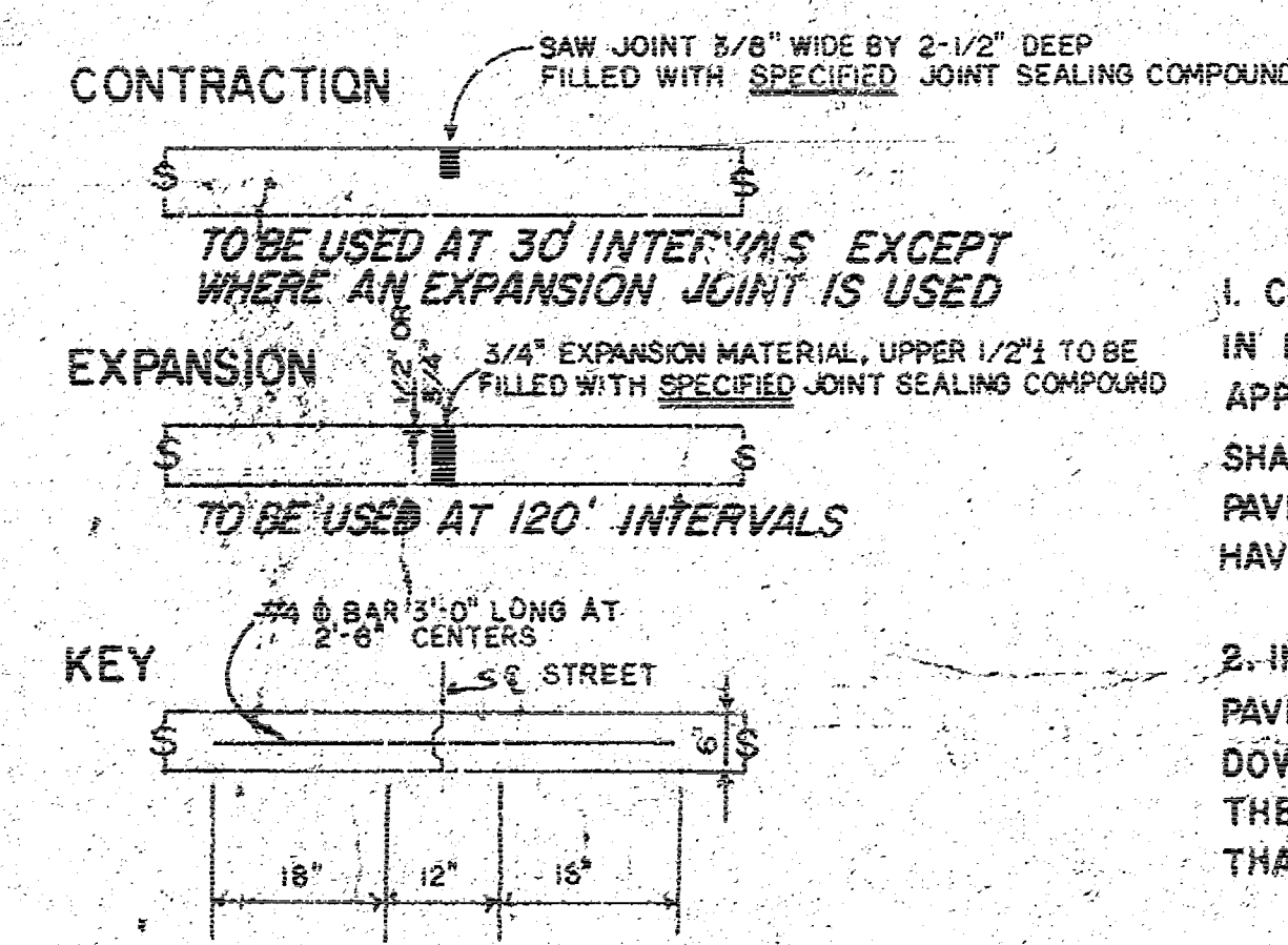
JOINT DETAILS
