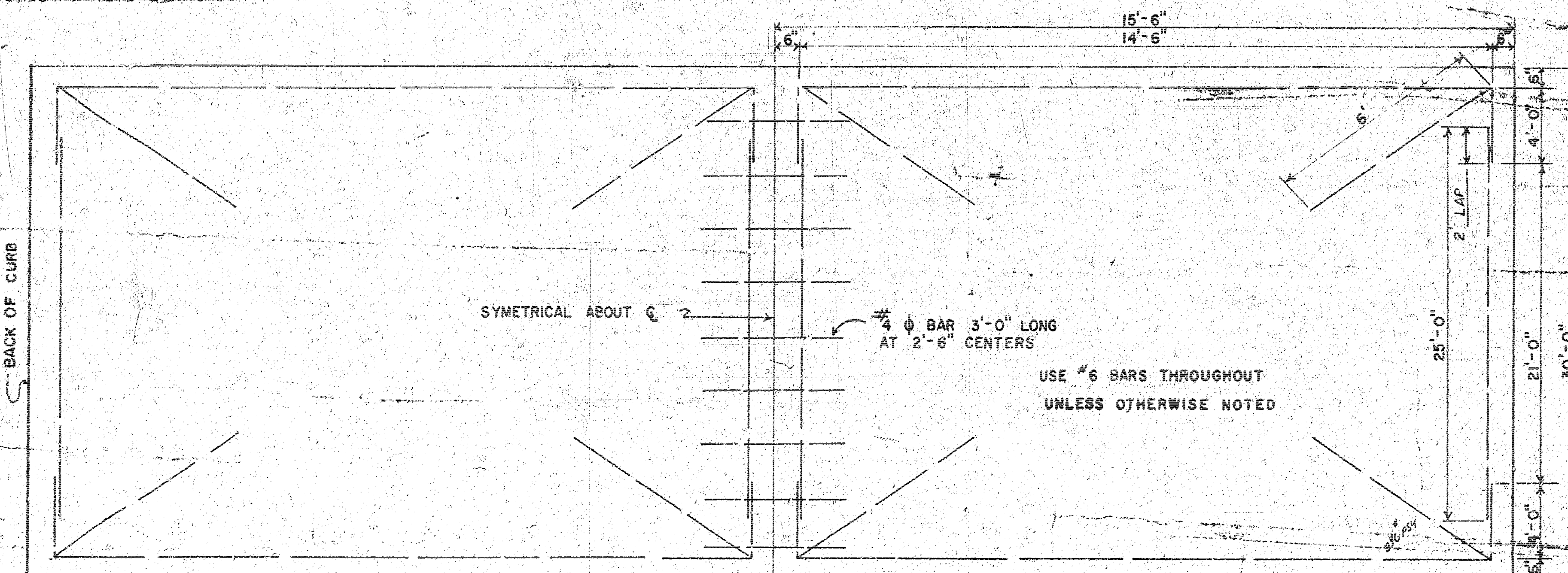
STEEL PATTERN
