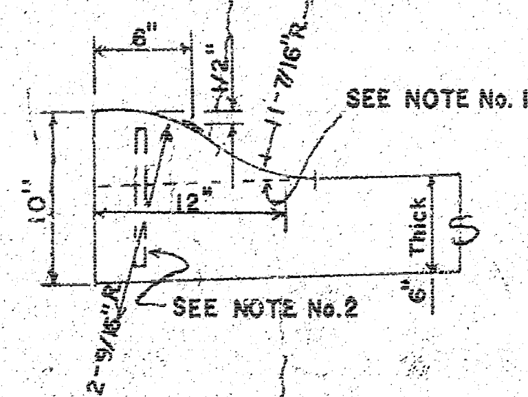
ALTERNATE ROLL-TYPE
