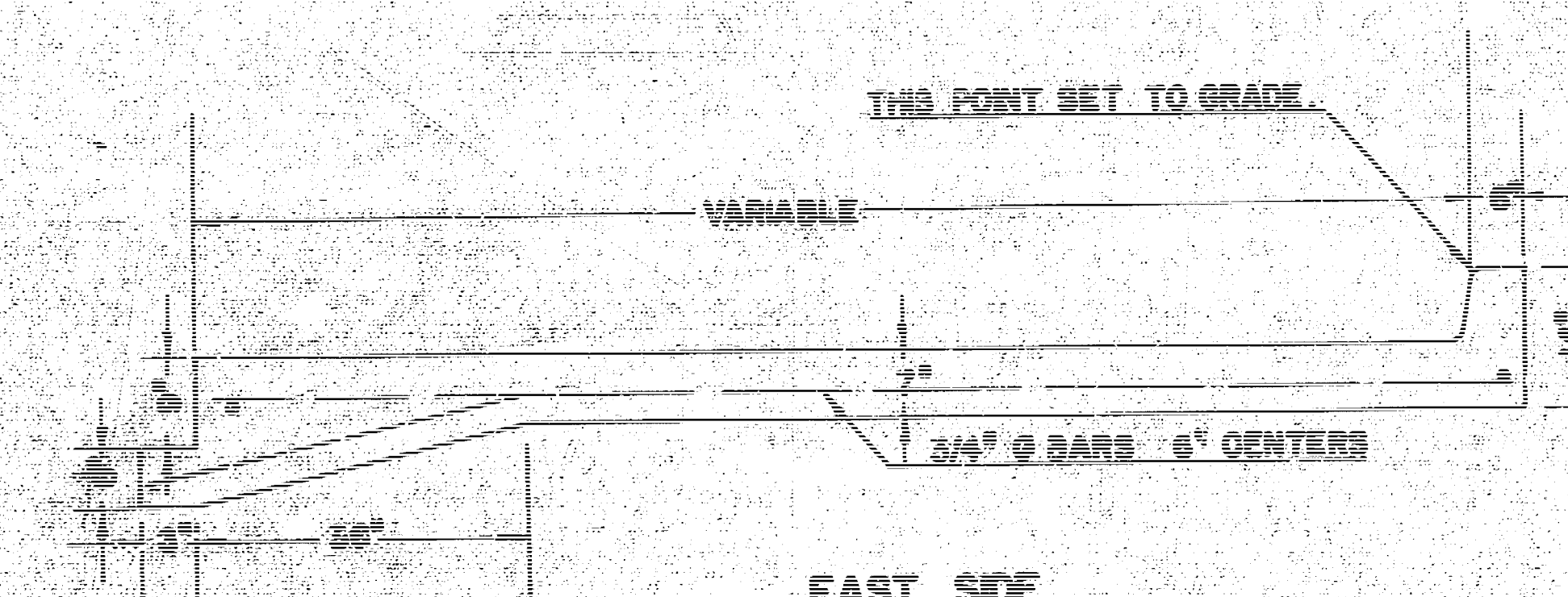
EAST SIDE 4+0 - N.L. STAFFORD TYPE C
