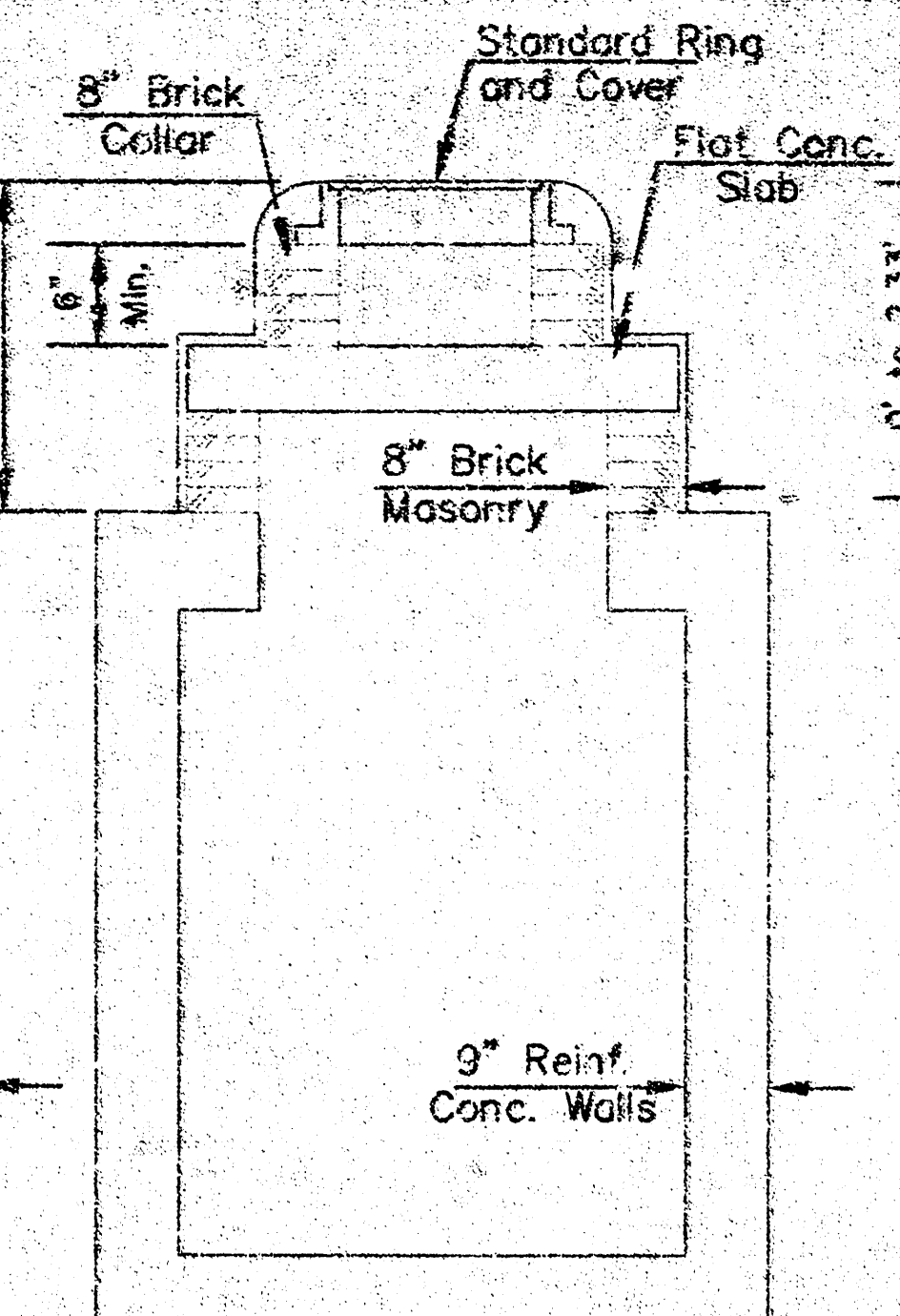
TYPE 3 Reinforced Concrete
