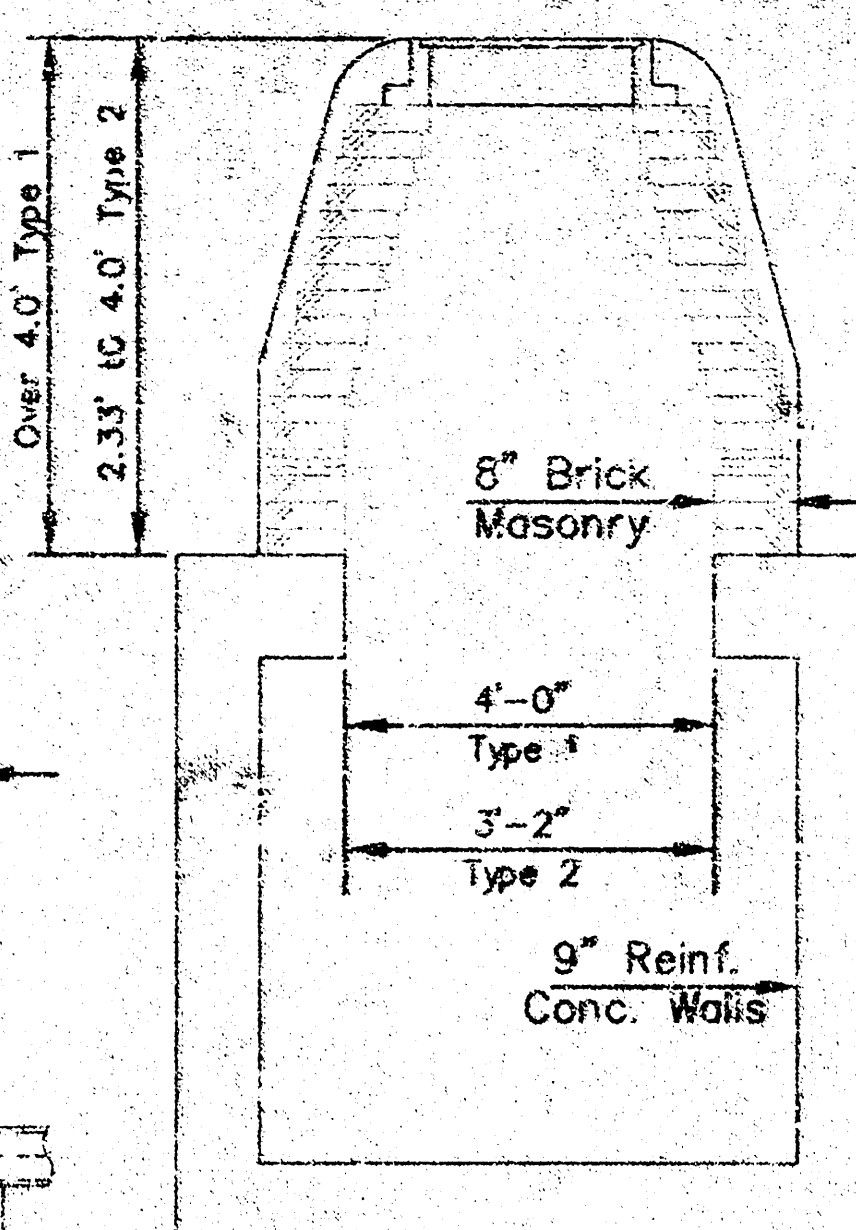
TYPE 1 & 2 Reinforced Concrete
