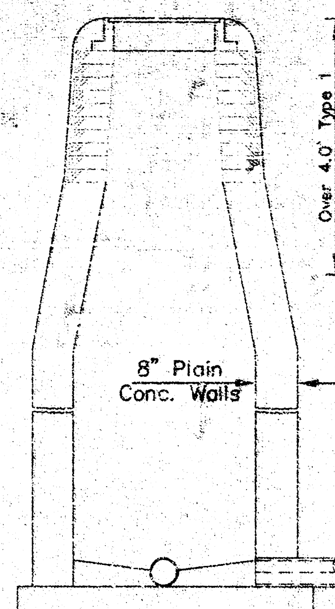
TYPE C & D Cast in Place (Type D is plastic lined & has brick araw)
