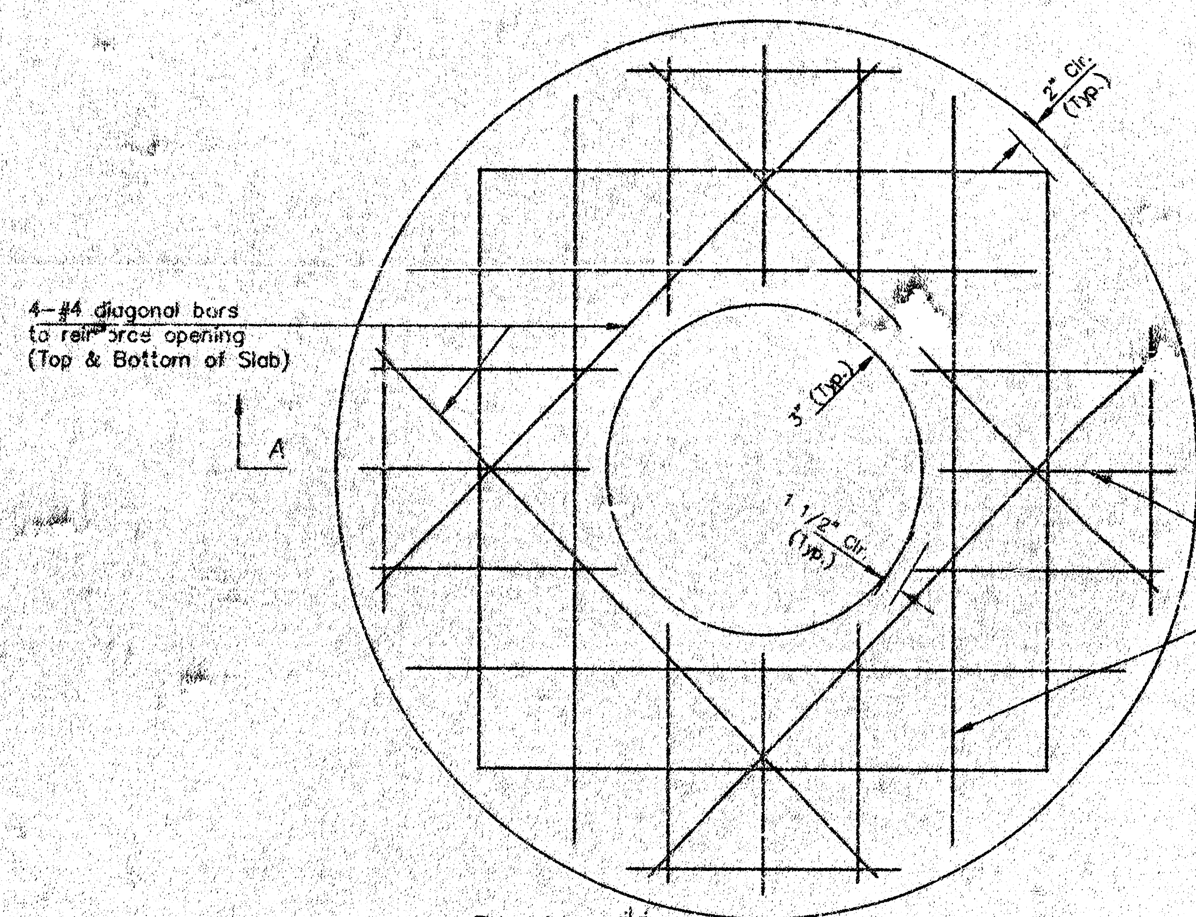
TYPE 4 Reinforced Concrete (Wide Flange Ring)
