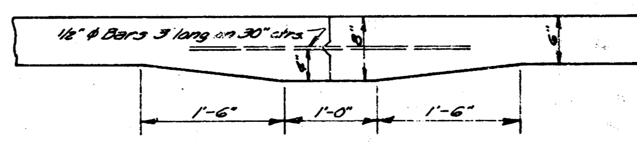
Mastic Joint Detail No Scale
