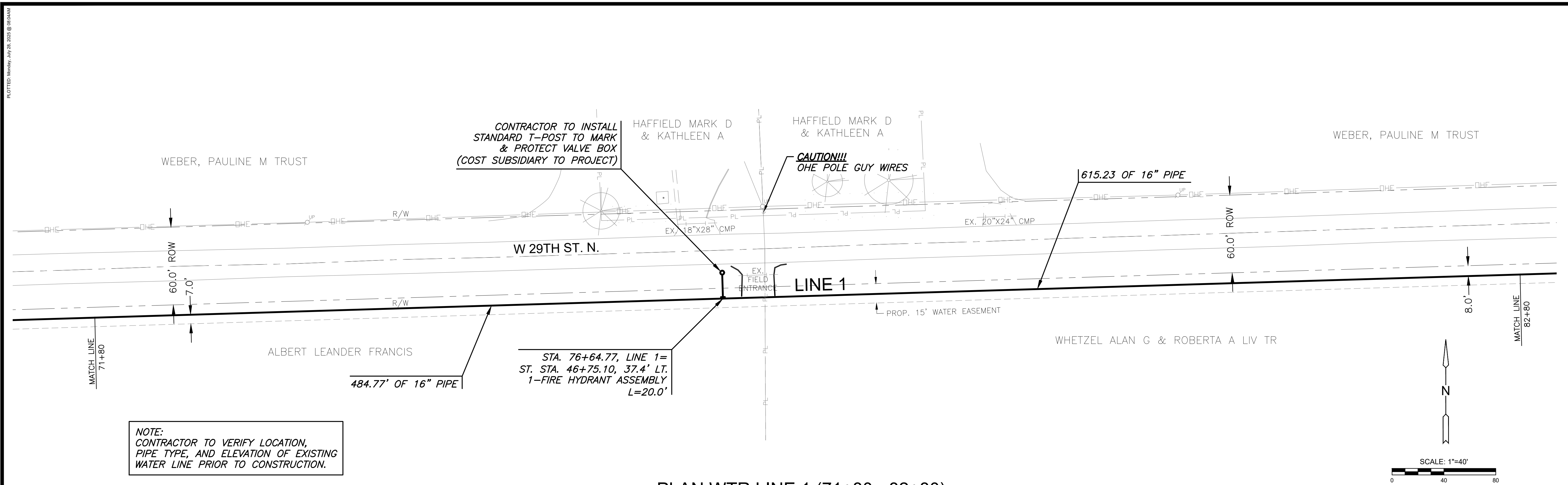
PLAN WTR LINE 1 (71+80 - 82+80) PROFILE WTR LINE 1 (71+80 - 82+80)
