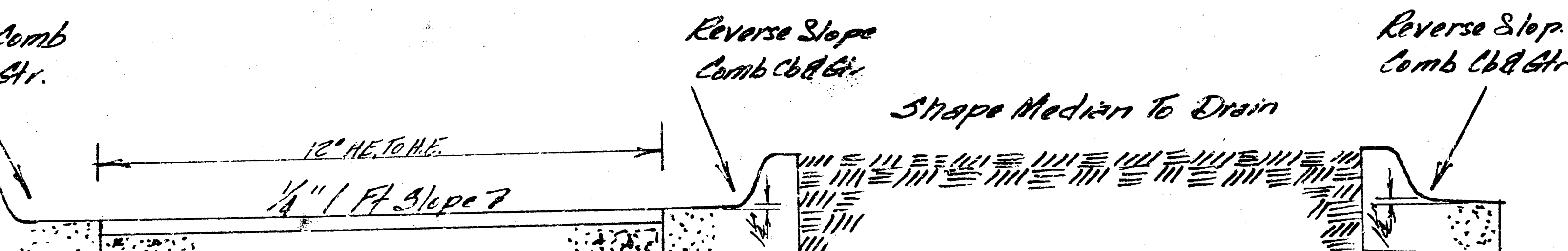
TYPICAL HALF SECTION No Scale
