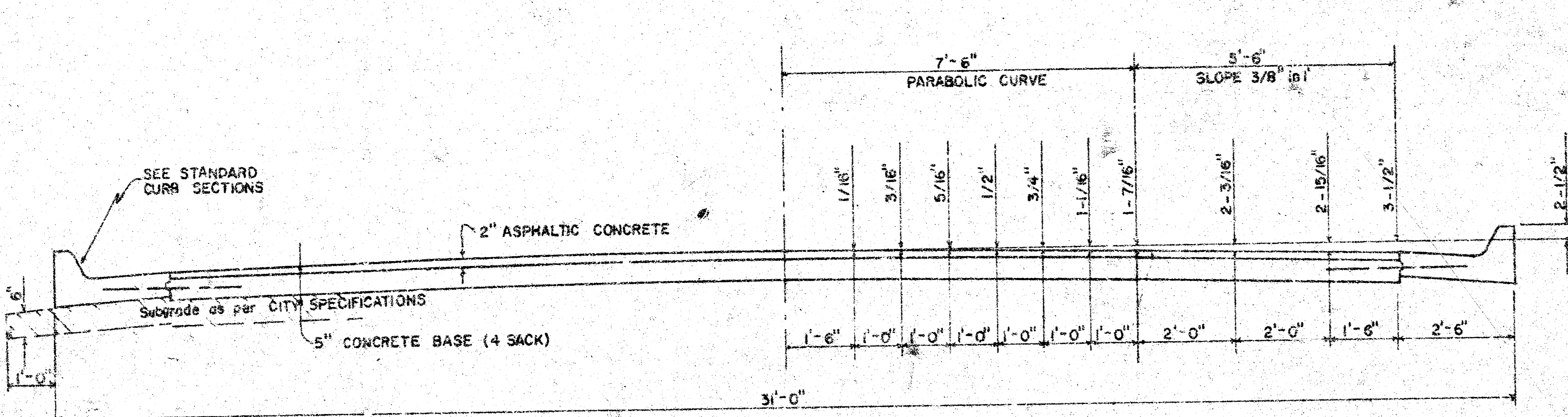
TYPICAL SECTION WITH STANDARD CROWN
