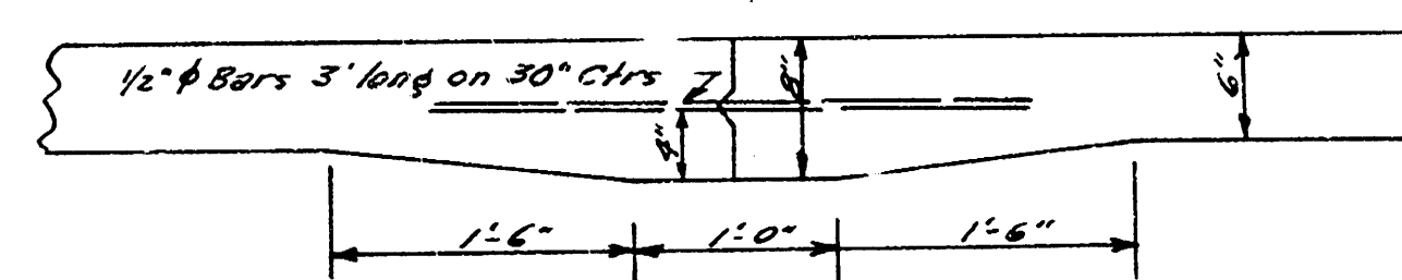
MASTIC JOINT DETAIL NO SCALE
