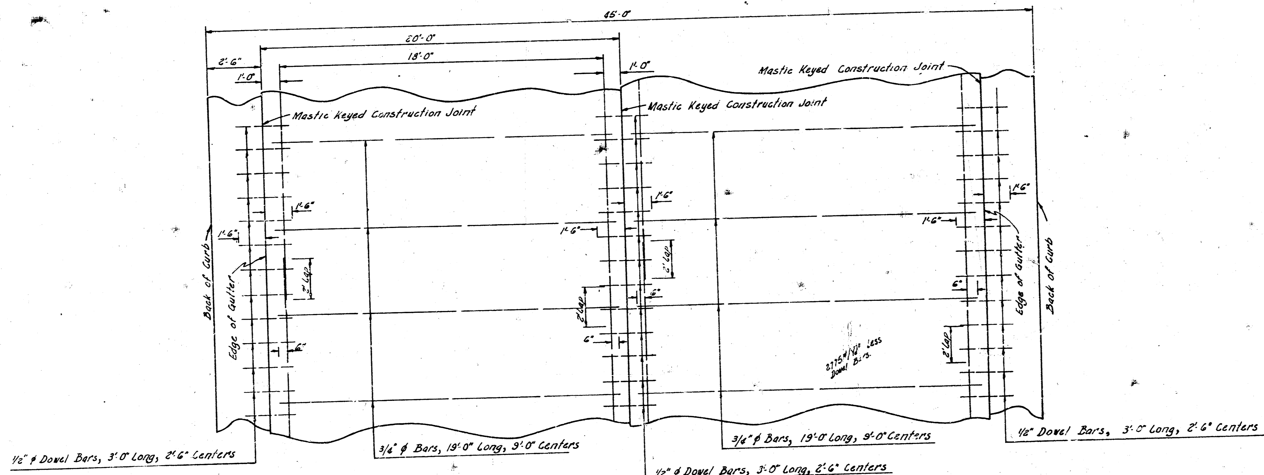
STEEL PATTERN NOT TO SCALE USE 3/4" Ø BARS EXCEPT WHERE NOTED
