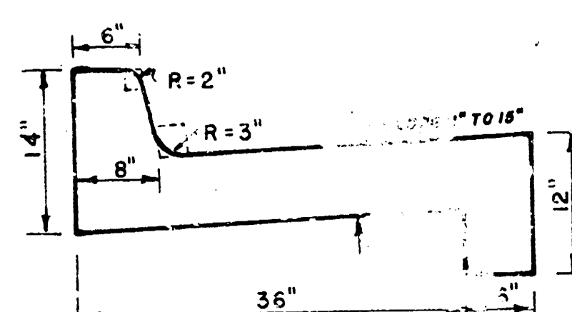
COMBINED CURB & GUTTER SECTION
