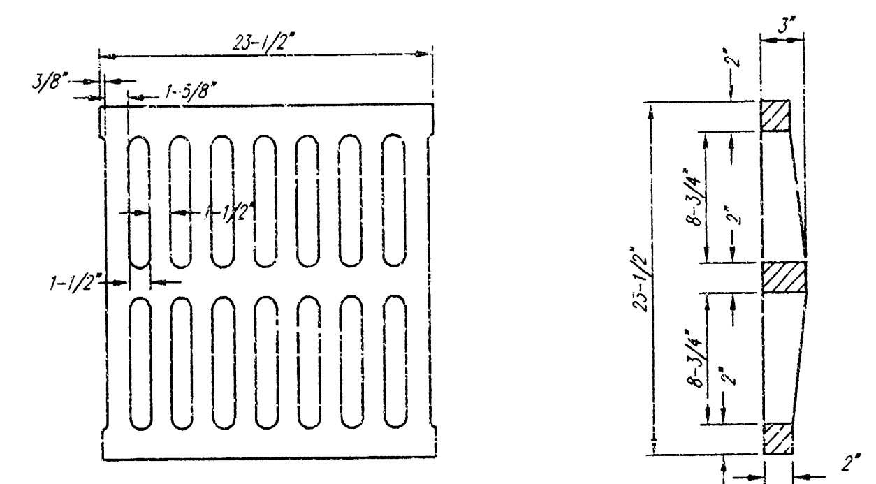
DEETER #2433 GRATE
