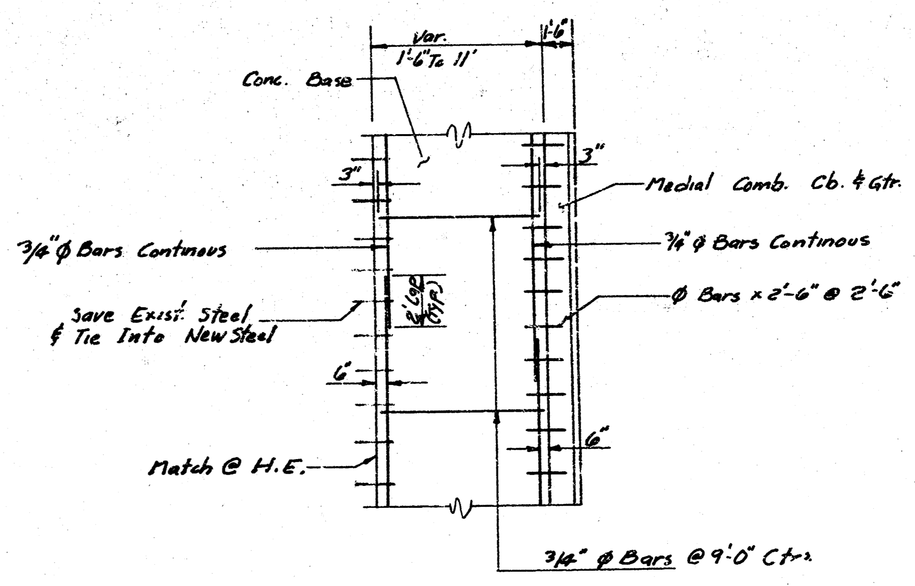
STEEL PATTERN CONC. BASE
