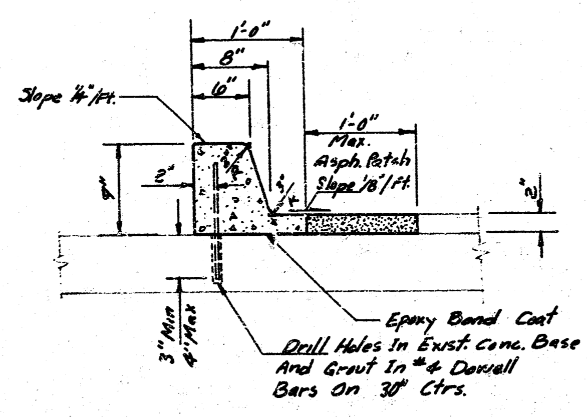
DOWELLED MEDIAL CURB
