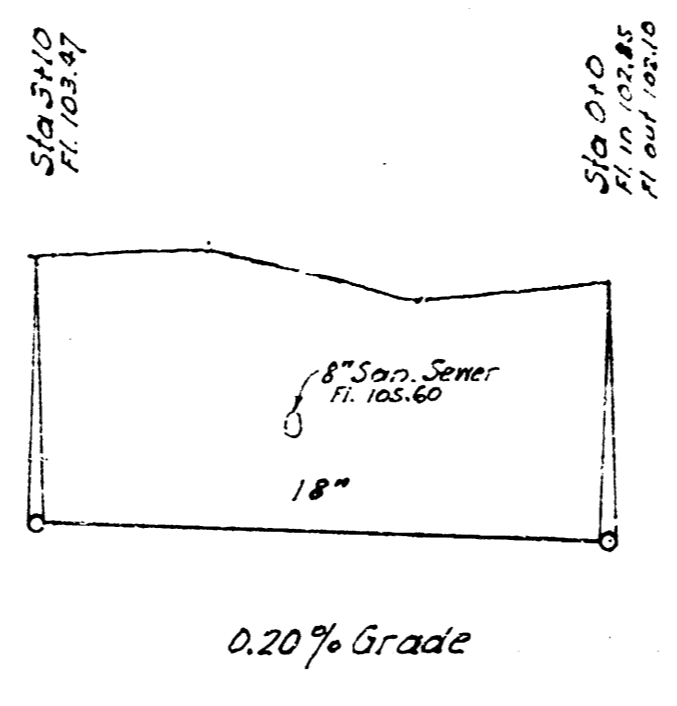
PROFILE OF LINE #3
