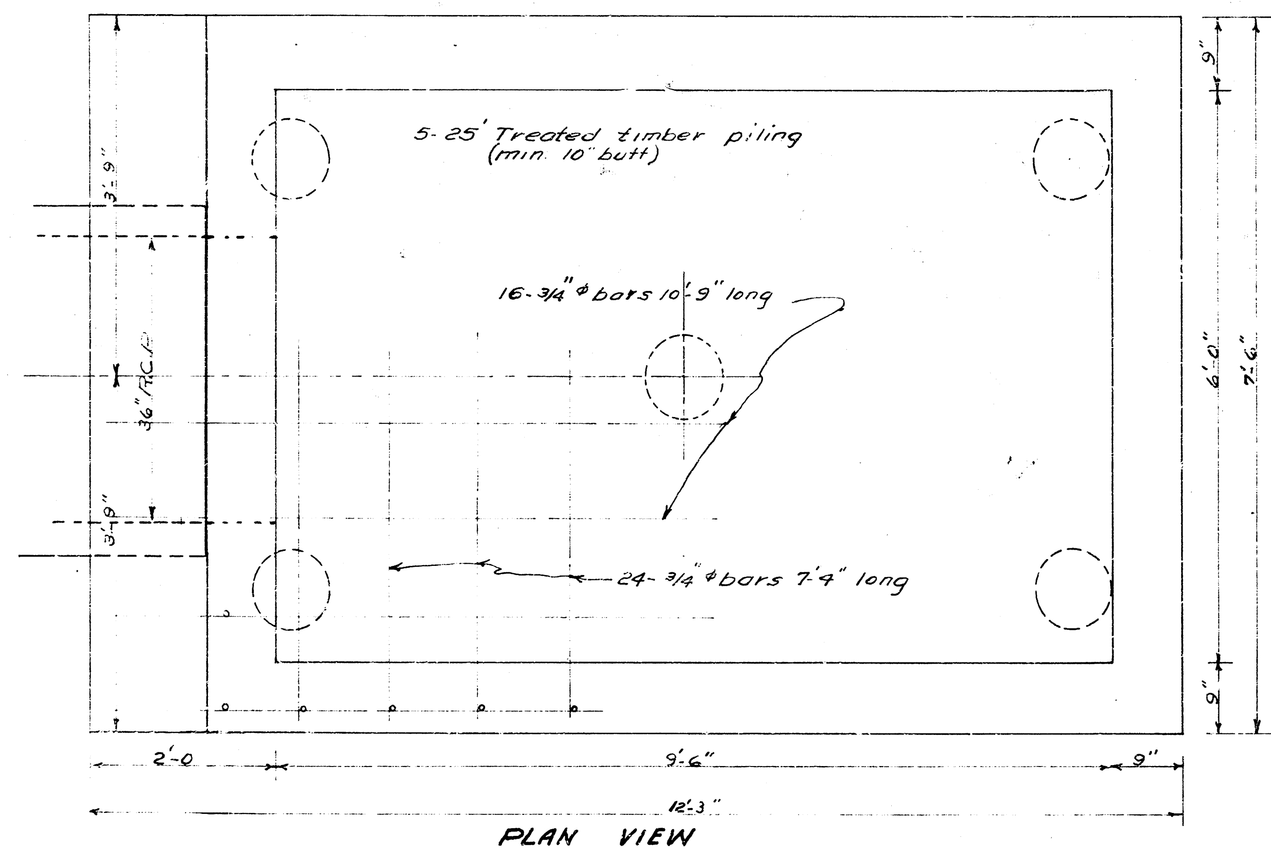
REINF. CONCRETE OUTFALL STRUCTURE Scale 1"=1'-0"
