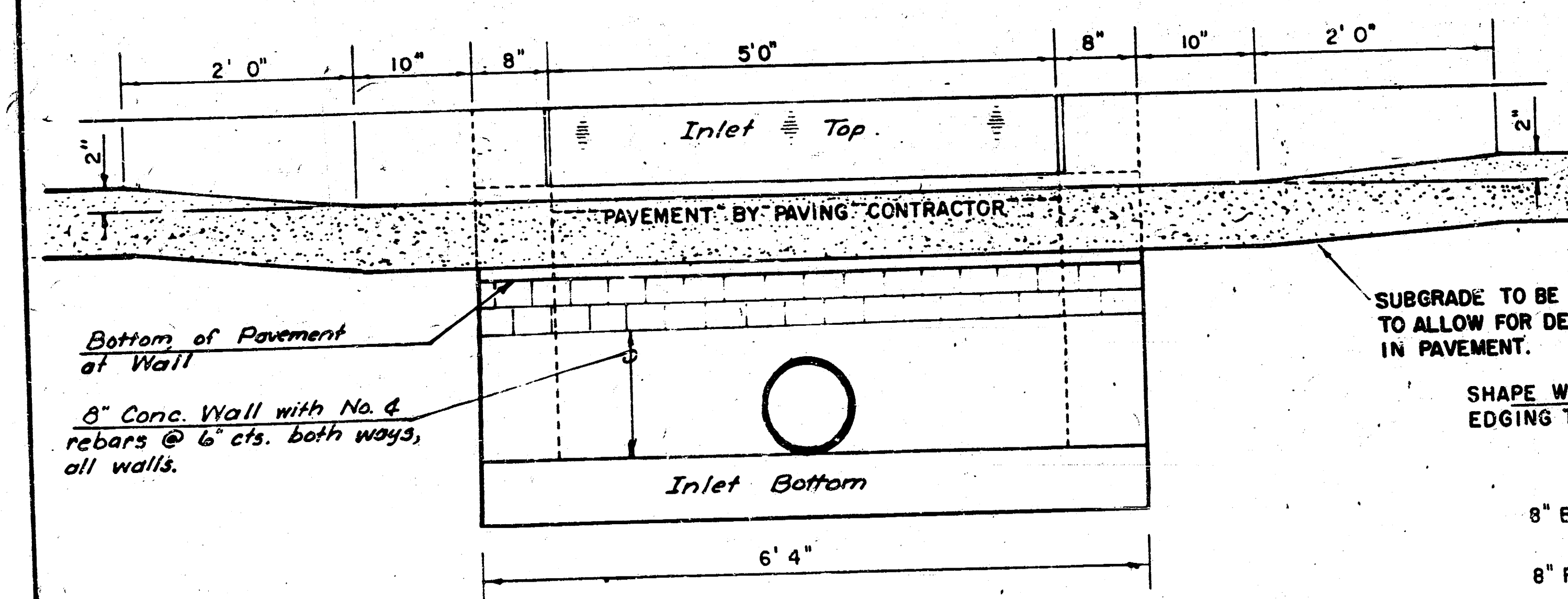
SECTION C-C
