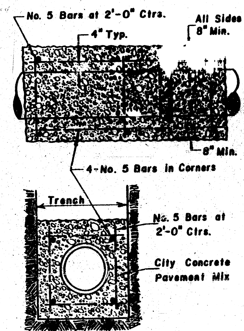
Detail Of Reinforced Concrete Encasement
