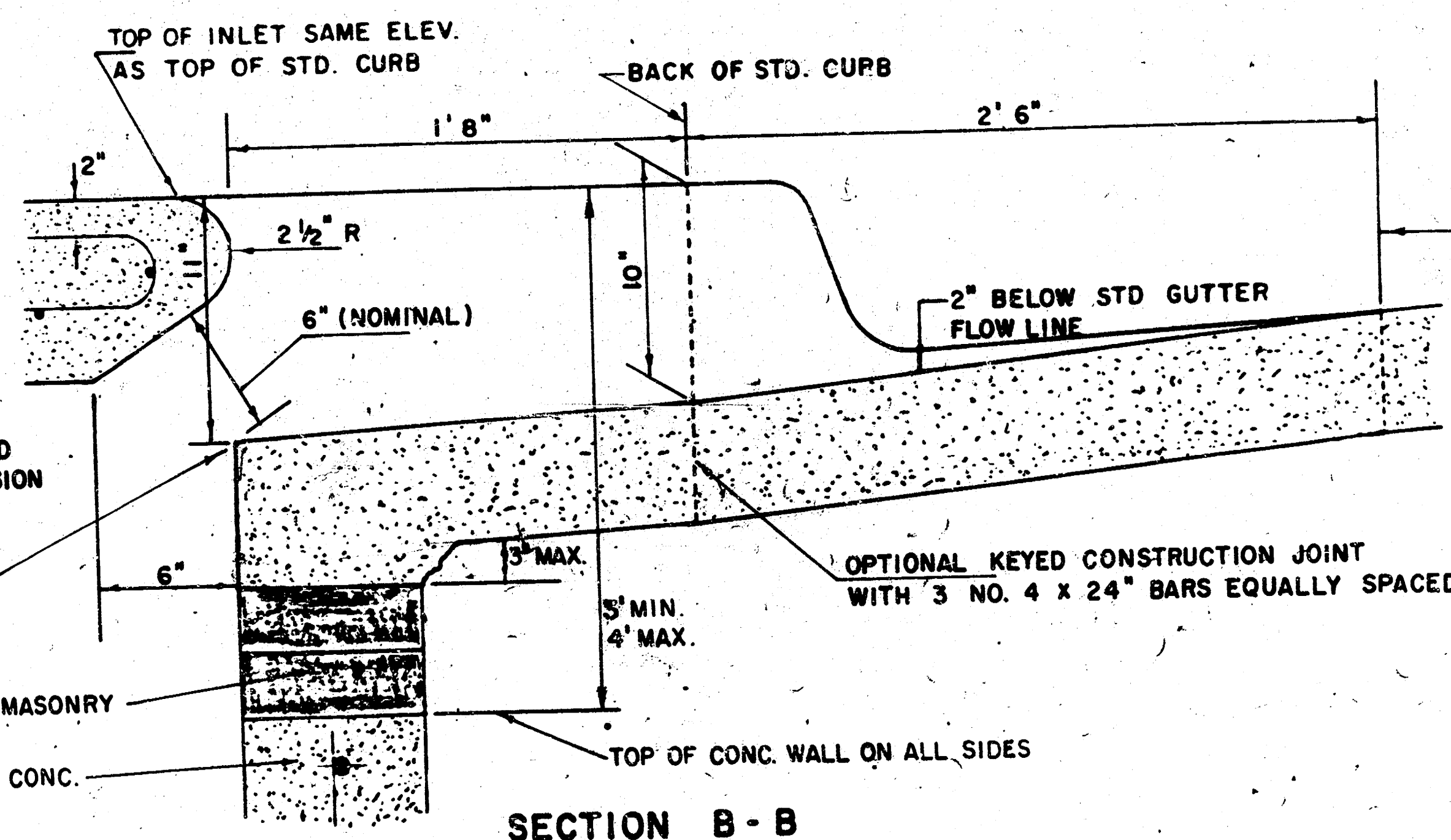
SECTION B-B
