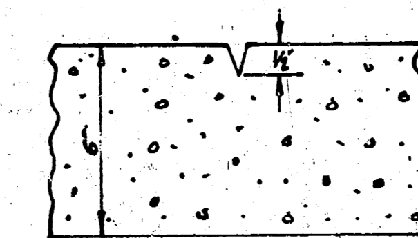
DETAIL - PLANE OF WEAKNESS PLANE OF WEAKNESS TO BE CUT WITH DOVEL-BASE, DEGREE TO DEPTH AS SHOWN IN A STRAIGHT LINE FROM CURB TO CURB. 26" CTR. TO CTR.
