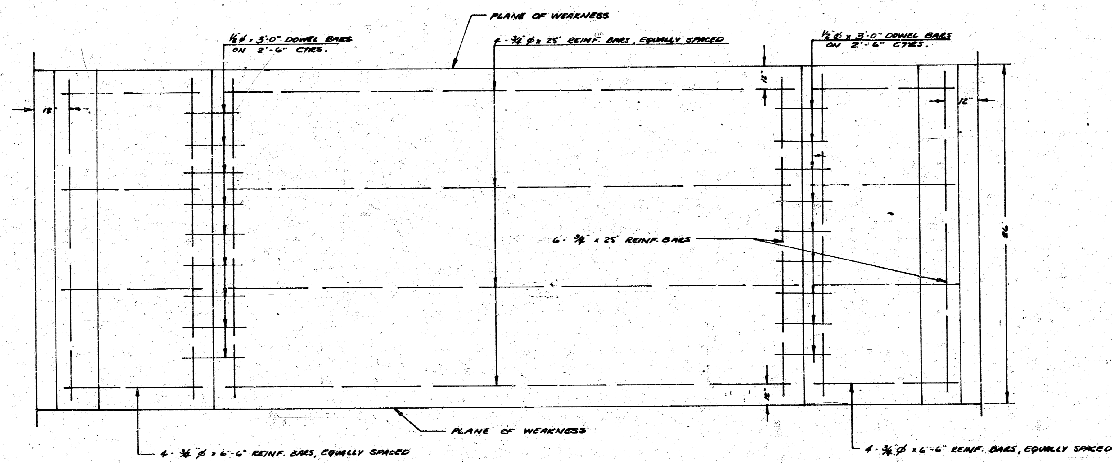
DETAIL - PLANE OF WEAKNESS PLANE OF WEAKNESS TO BE CUT WITH DOVEL-BASE, DEGREE TO DEPTH AS SHOWN IN A STRAIGHT LINE FROM CURB TO CURB. 26" CTR. TO CTR.
