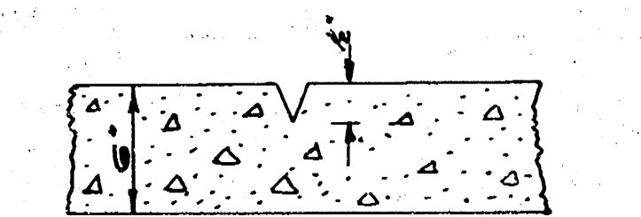
PLANE OF WEAKNESS DETAIL Plane of weakness to be cut with a double edged groove in a straight line from curb to curb on 26' centers.
