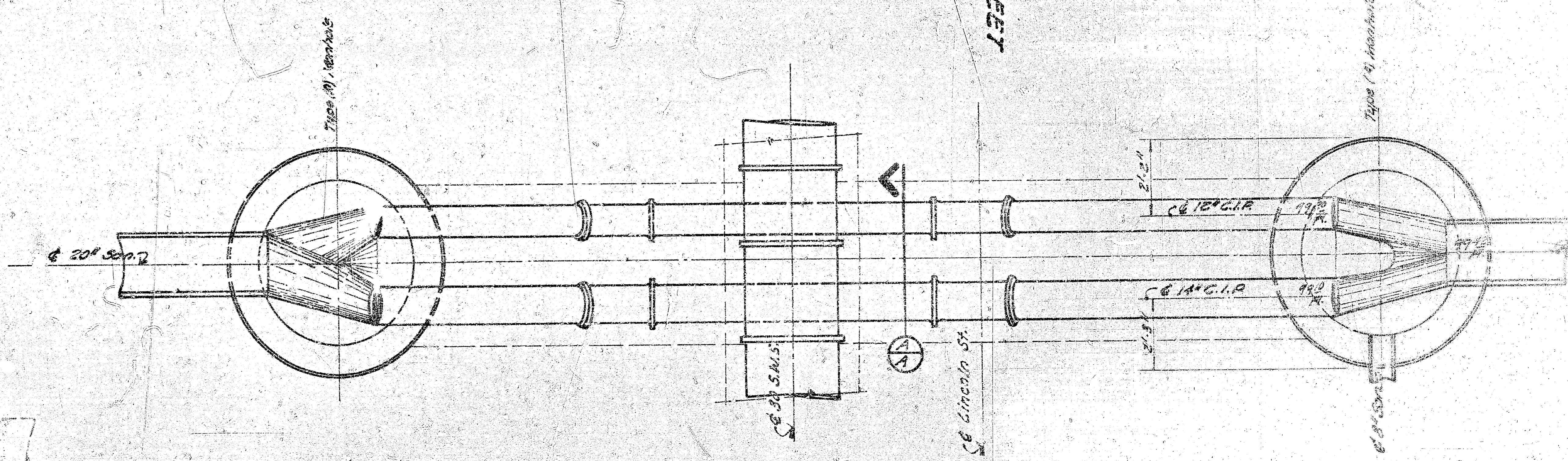
SANITARY SEWER SIPHON DETAIL (Sta. 13+43.2)
