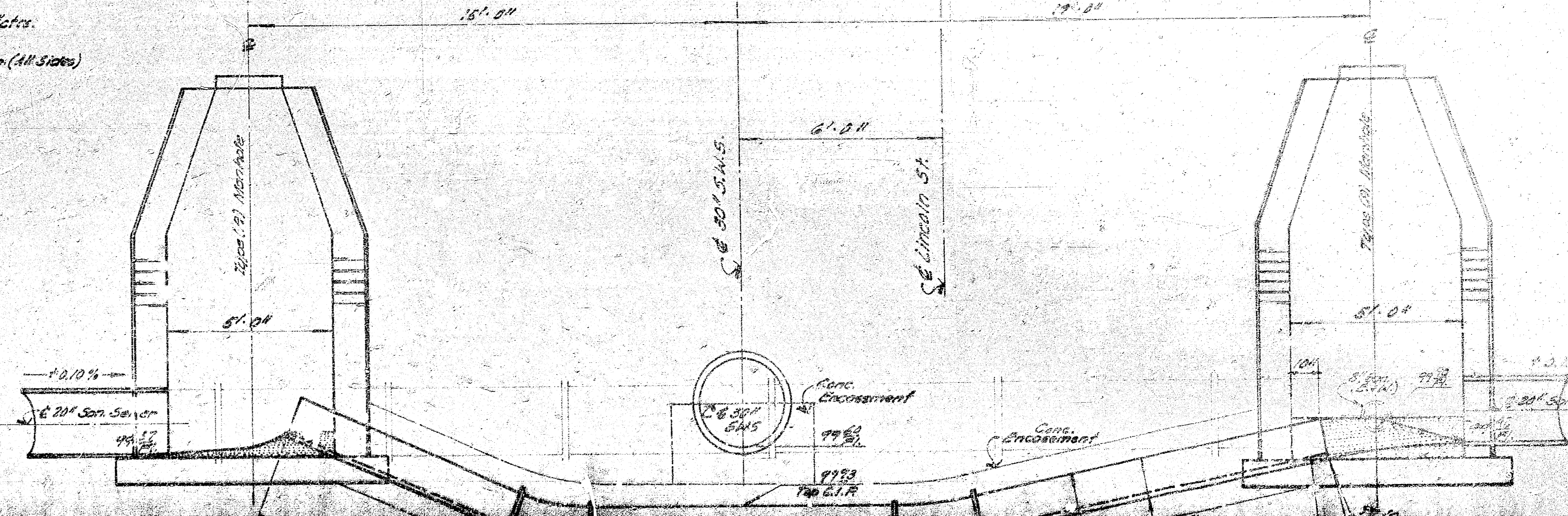
SANITARY SEWER SIPHON DETAIL (Sta. 13+43.2)
