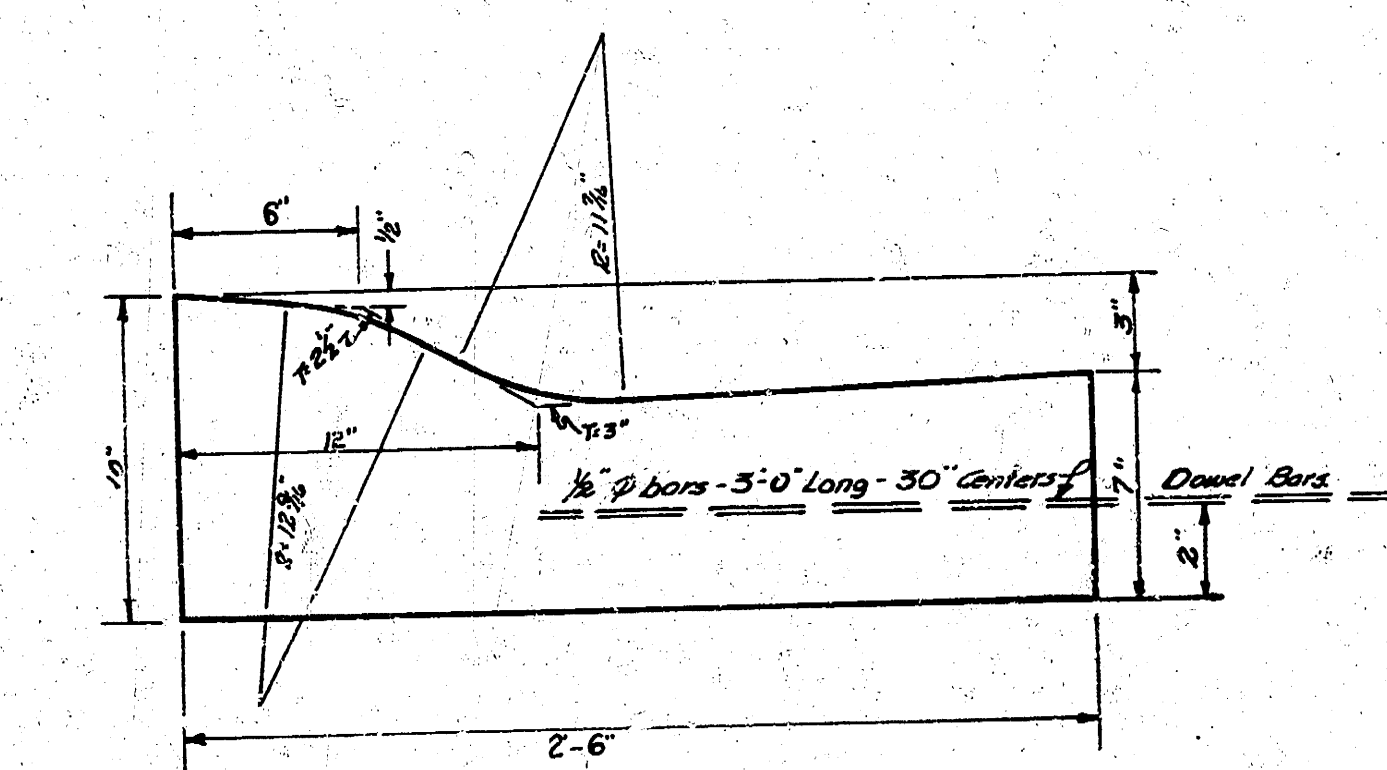
NON-STD. COMB. CURB & GUTTER DETAIL To be poured with 3 sack concrete mix. SCALE: 2" = 1'-0"
