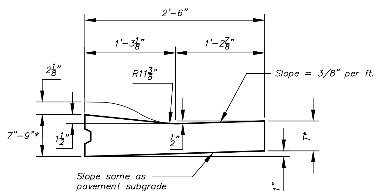
Combined Curb & Gutter (3 5/8")
