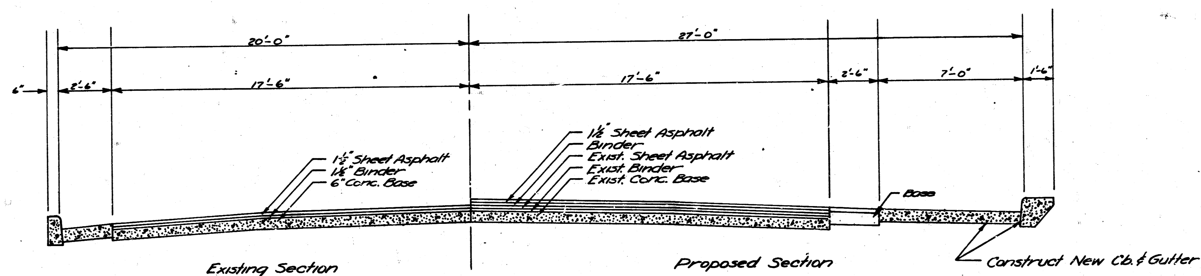
TYPICAL SECTION S.L. WATERMAN-N.L. LEWIS
