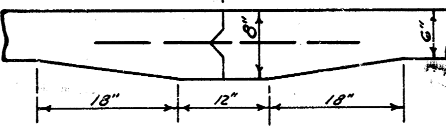
Use \frac{1}{2} " bars 3.0' long @ 30" cts. MASTIC JOINT DETAIL
