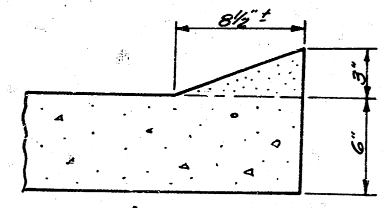
3" Monolithic Edge Curb No Scale Use where noted on plan.
