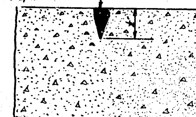
DETAIL OF PLANE OF WEAKNESS EVERY 4TH JOINT TO BE EXPANSION JOINT No Scale
