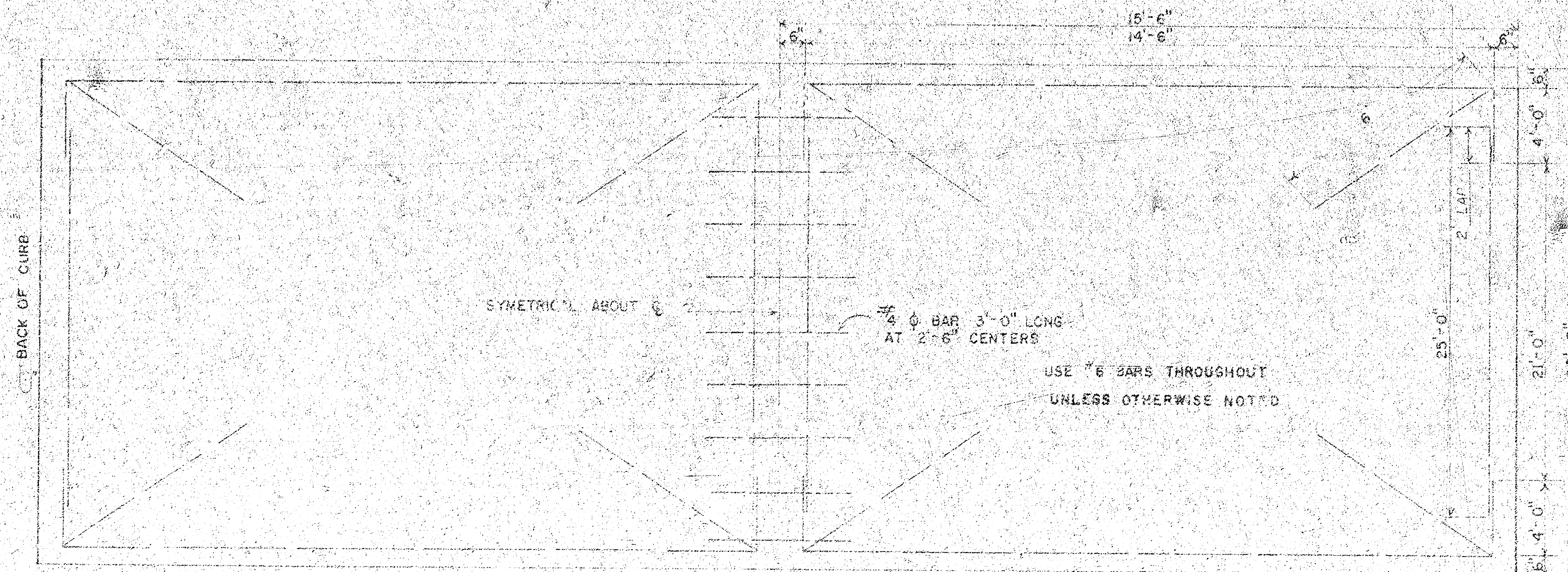
STEEL PATTERN
