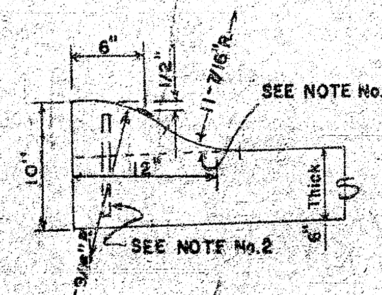
ALTERNATE ROLL-TYPE
