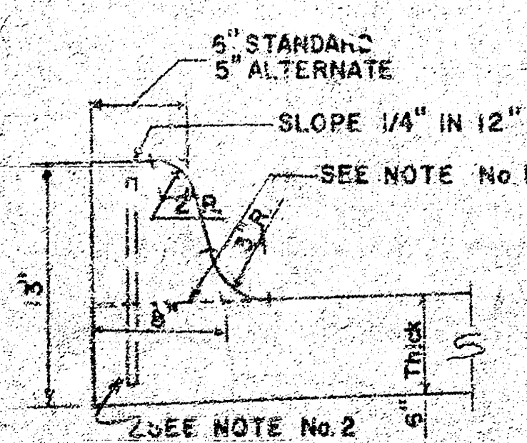
INTEGRAL CURB
