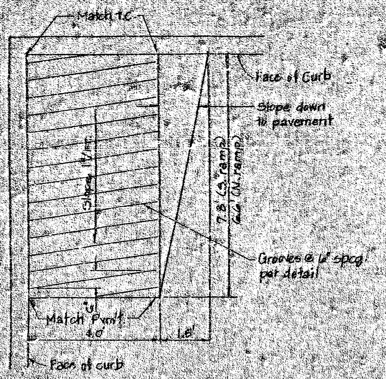
WHEELCHAIR RAMP DETAIL
