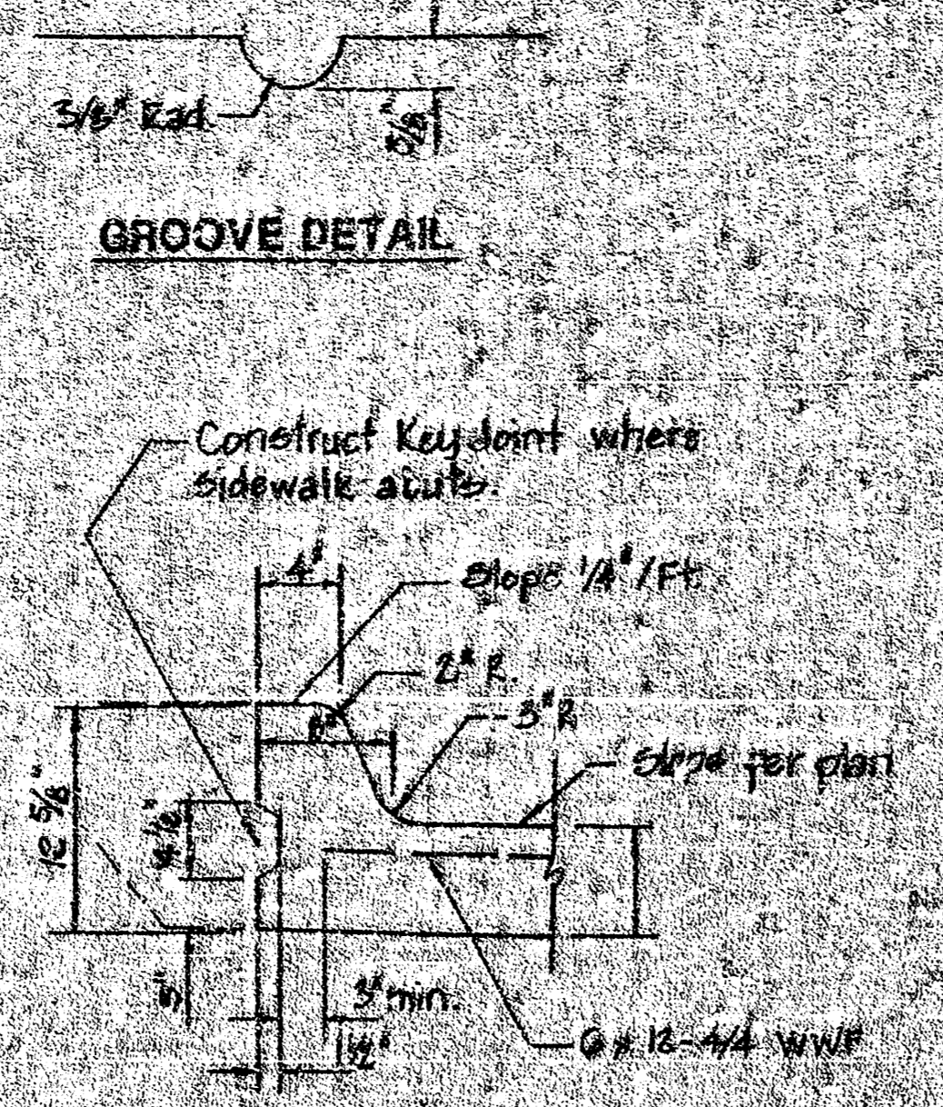
MONOLITHIC CURB DETAIL
