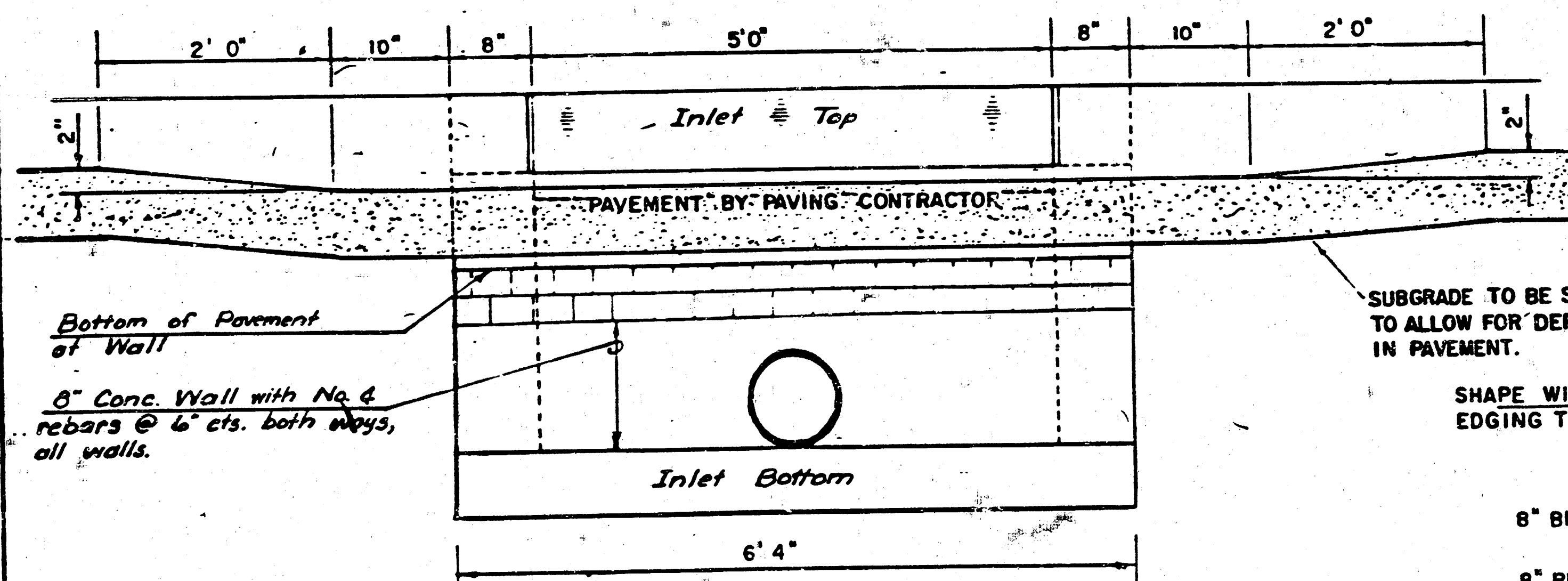
SECTION C-C
