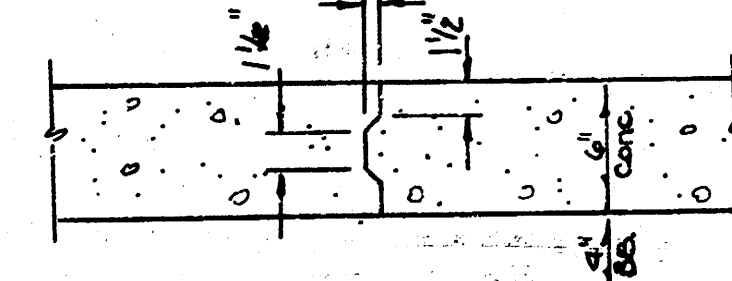
ALTERNATE LONGITUDINAL JOINT
