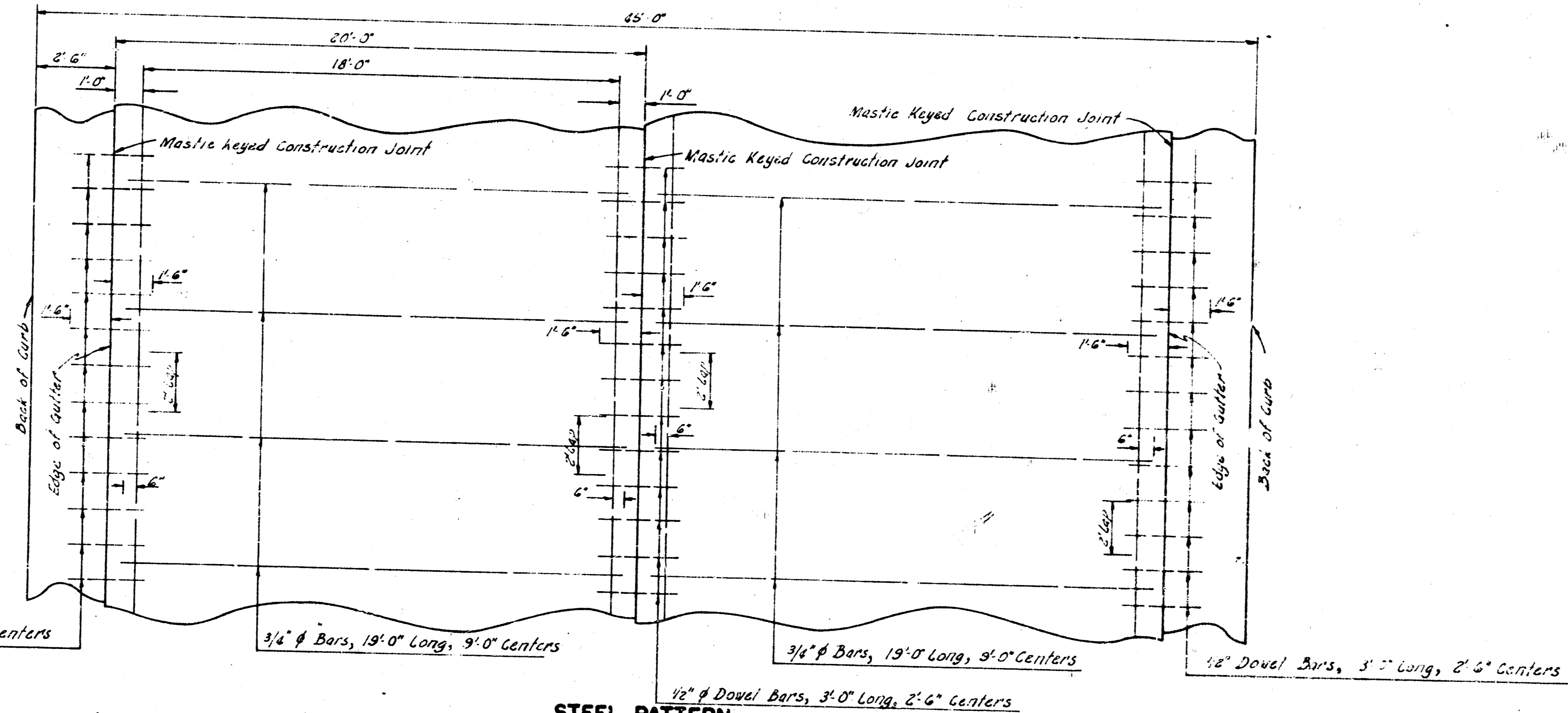
STEEL PATTERN
