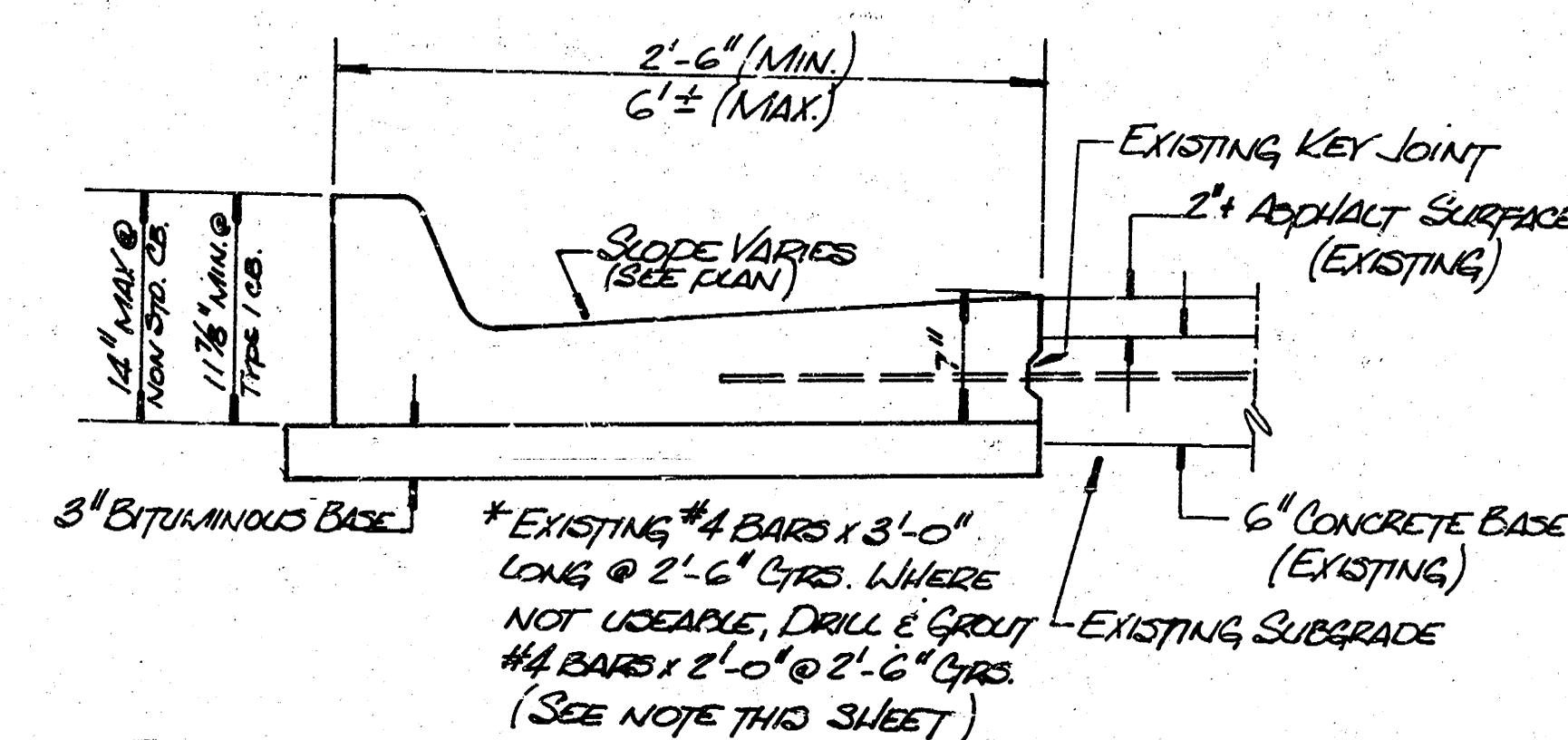
TRANSITION CURB & GUTTER
