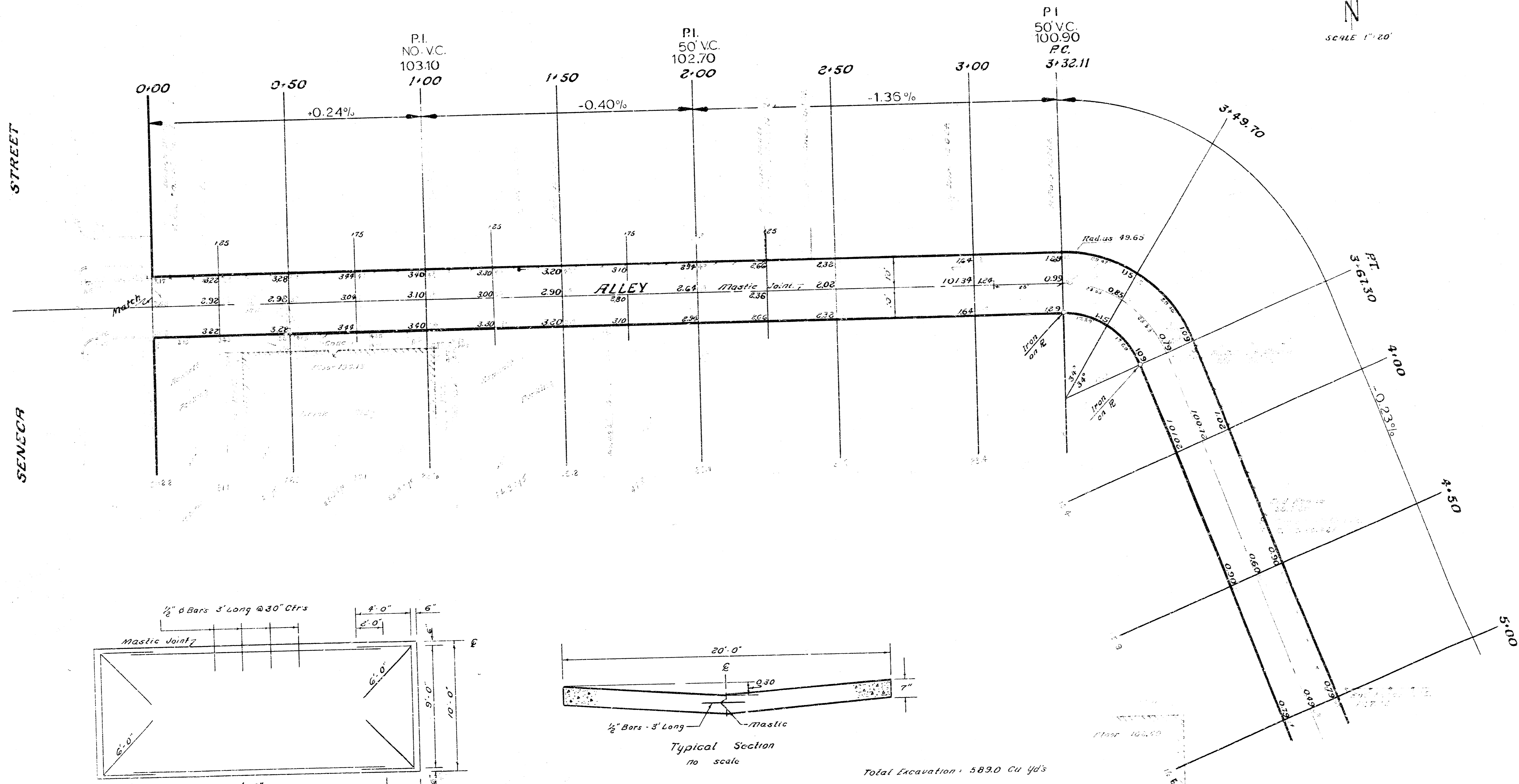
Steel Pattern All Steel to be 3/4" φ Except where shown.
