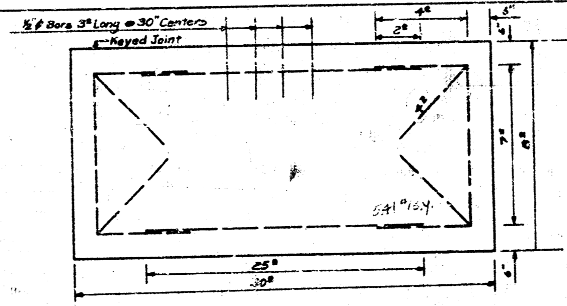
STEEL PATTERN No Scale All Steel to be 1/2" # Except Where Noted
