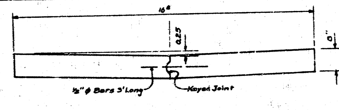
TYPICAL SECTION No Scale
