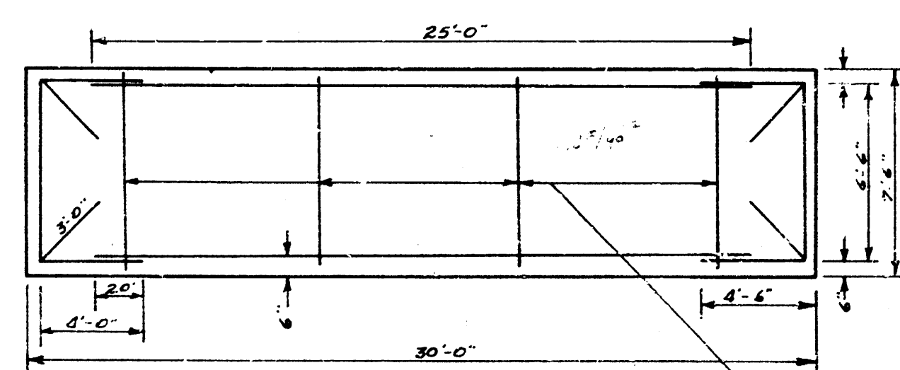
TYPICAL STEEL PATTERN No Scale
