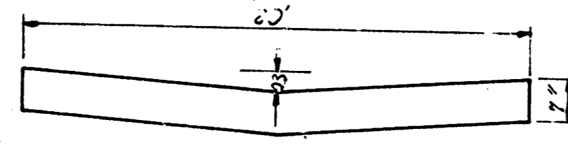
TYPICAL SECTION FROM STA 0+00 TO STA 4+00 NOT TO SCALE
