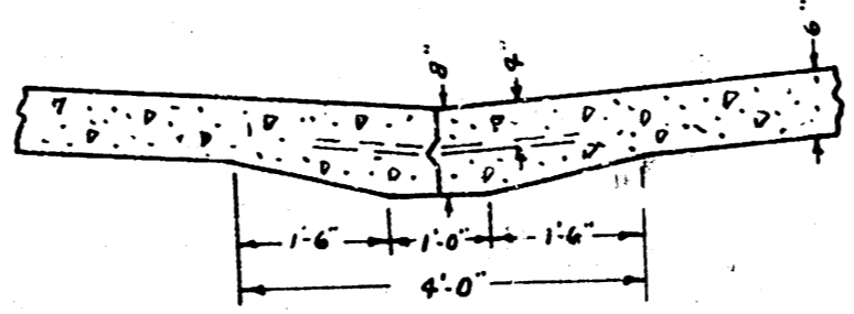
DETAIL OF MASTIC KEY JOINT
