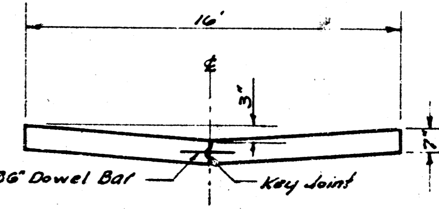
TYPICAL SECTION No Scale:
