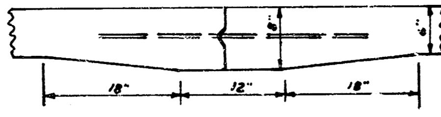
DETAILS OF MASTIC JOINT
