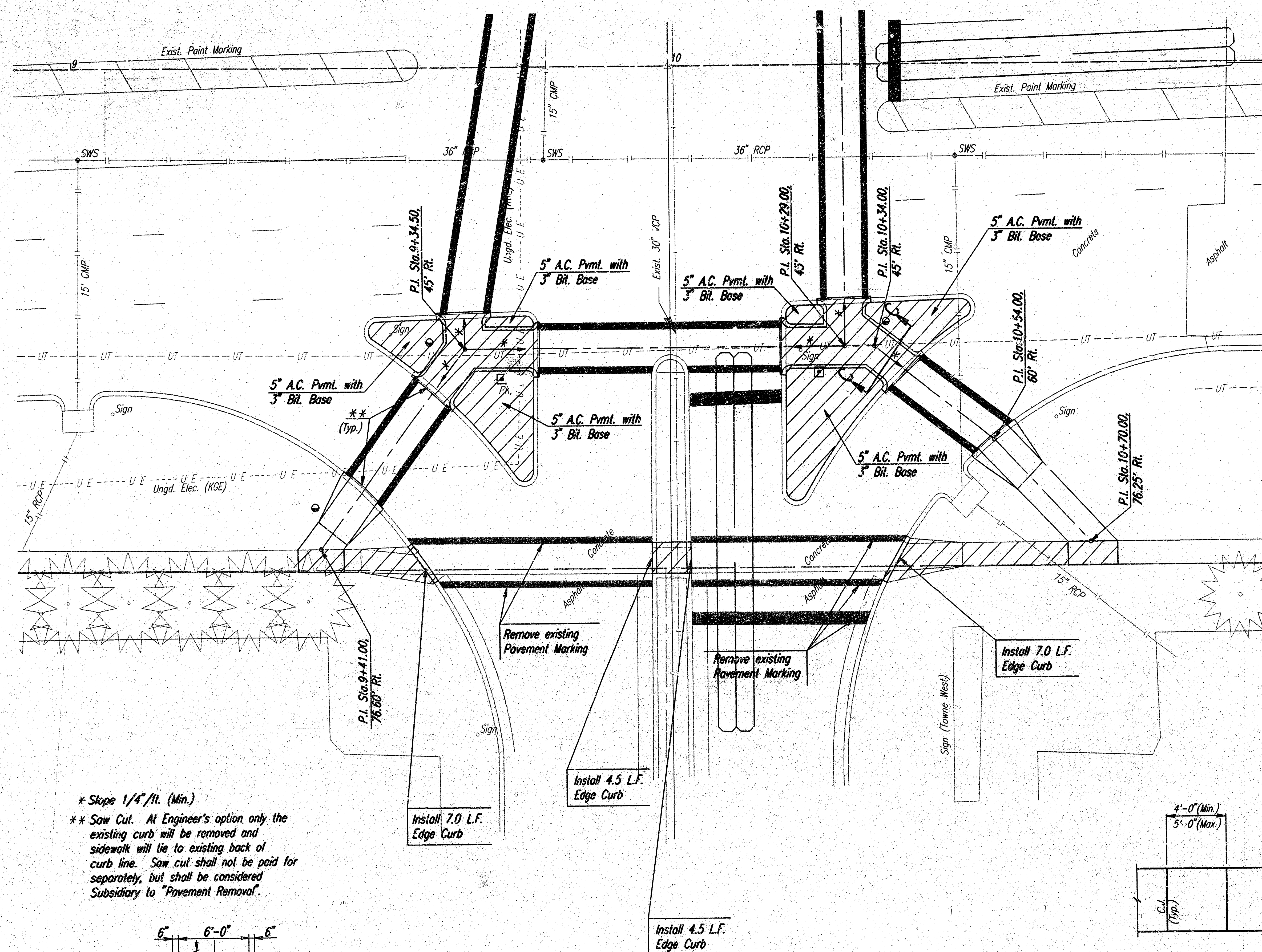
PLAN
