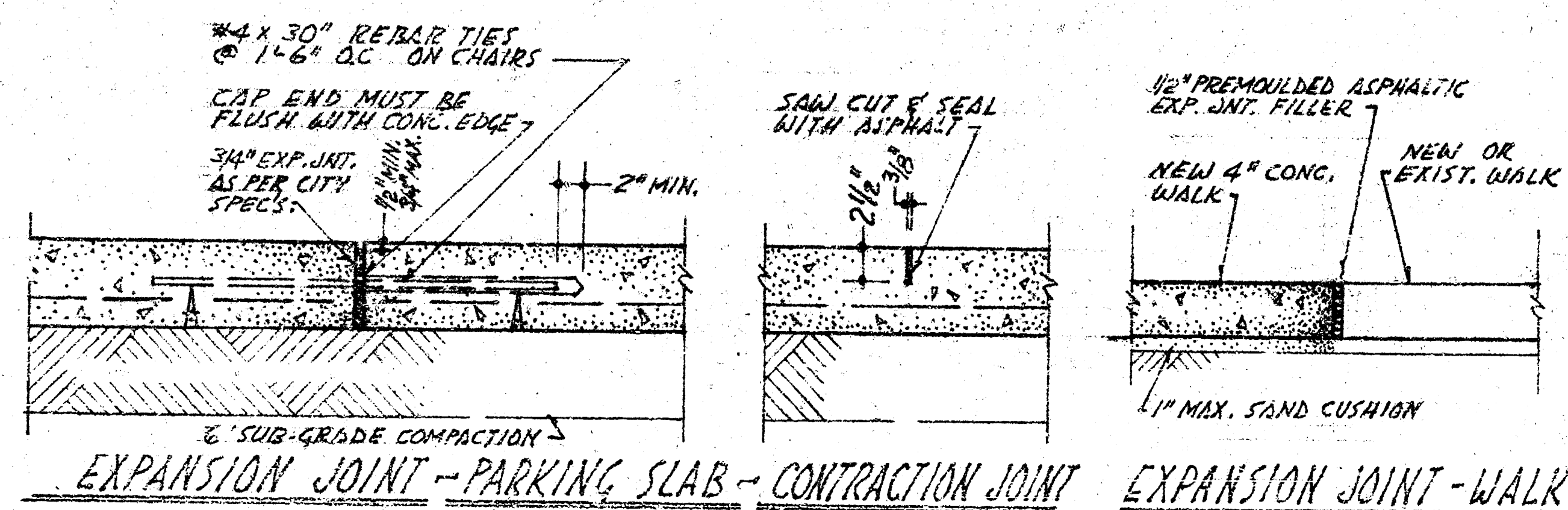
SLAB DETAILS HYDE ELEMENTARY SCALE - 1" = 1'-0"
