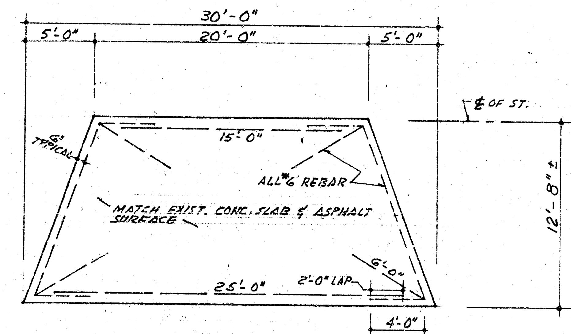
REBAR PLACEMENT PLAN FRANKLIN ELEMENTARY SCALE - 1" = 60'-0"
