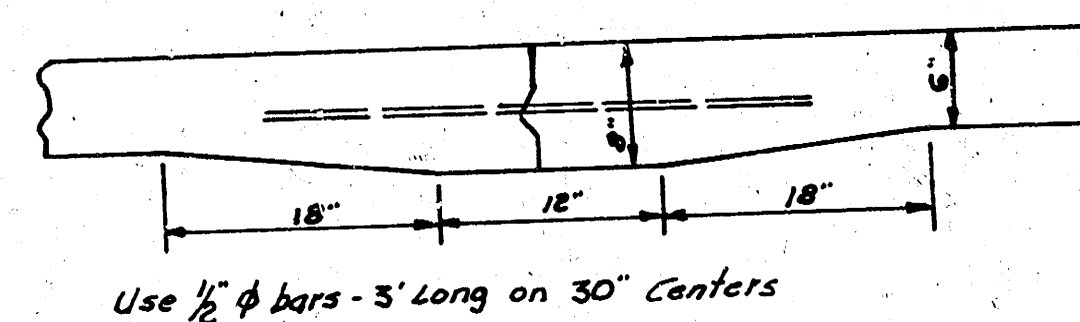
Use \frac{1}{2} " \phi bars - 5' long on 30" Centers No Scale.
