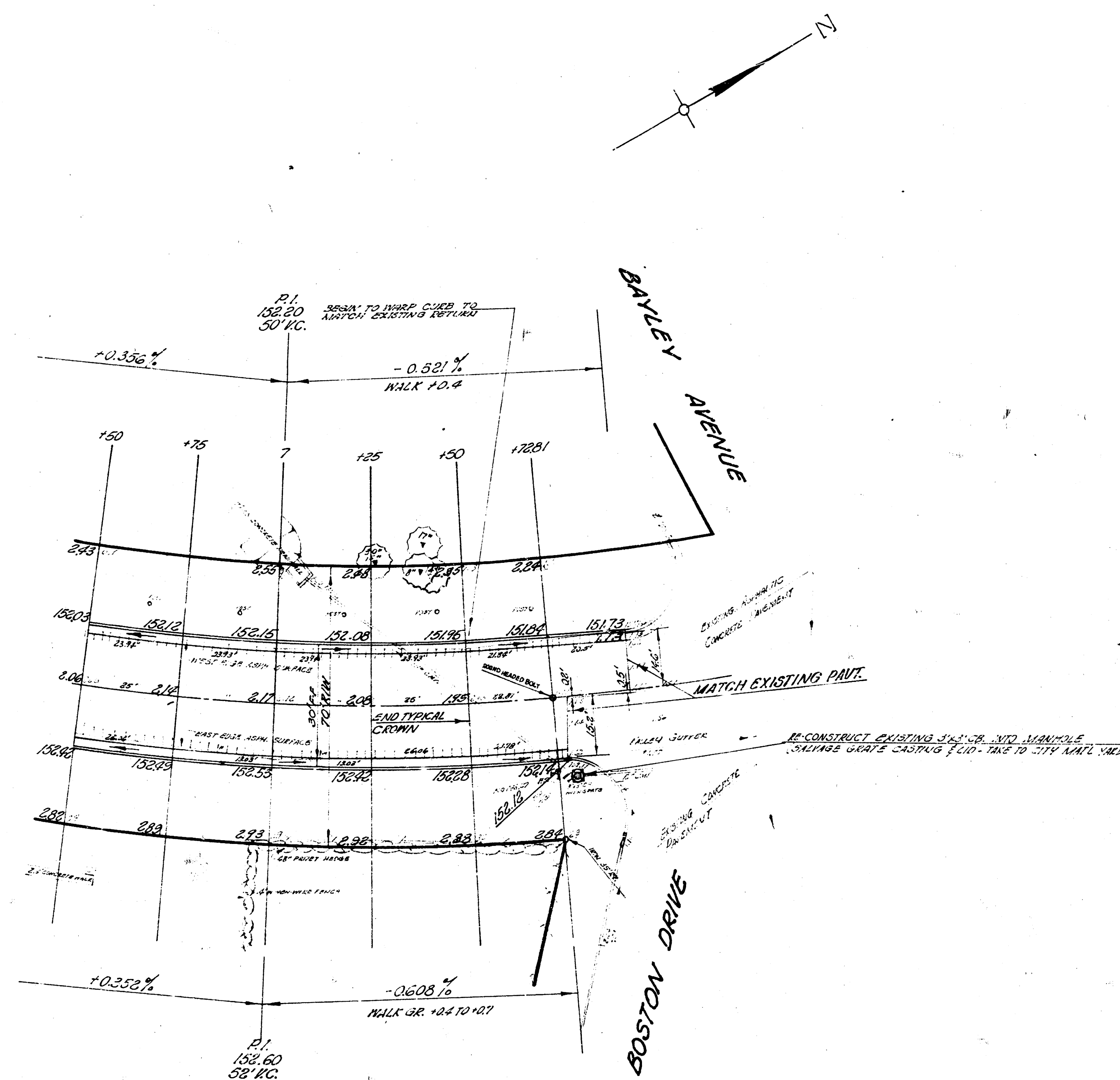
CURVE DATA BASED ON Q RADIUS = 500.15' \Delta = 18^{\circ} 20'
