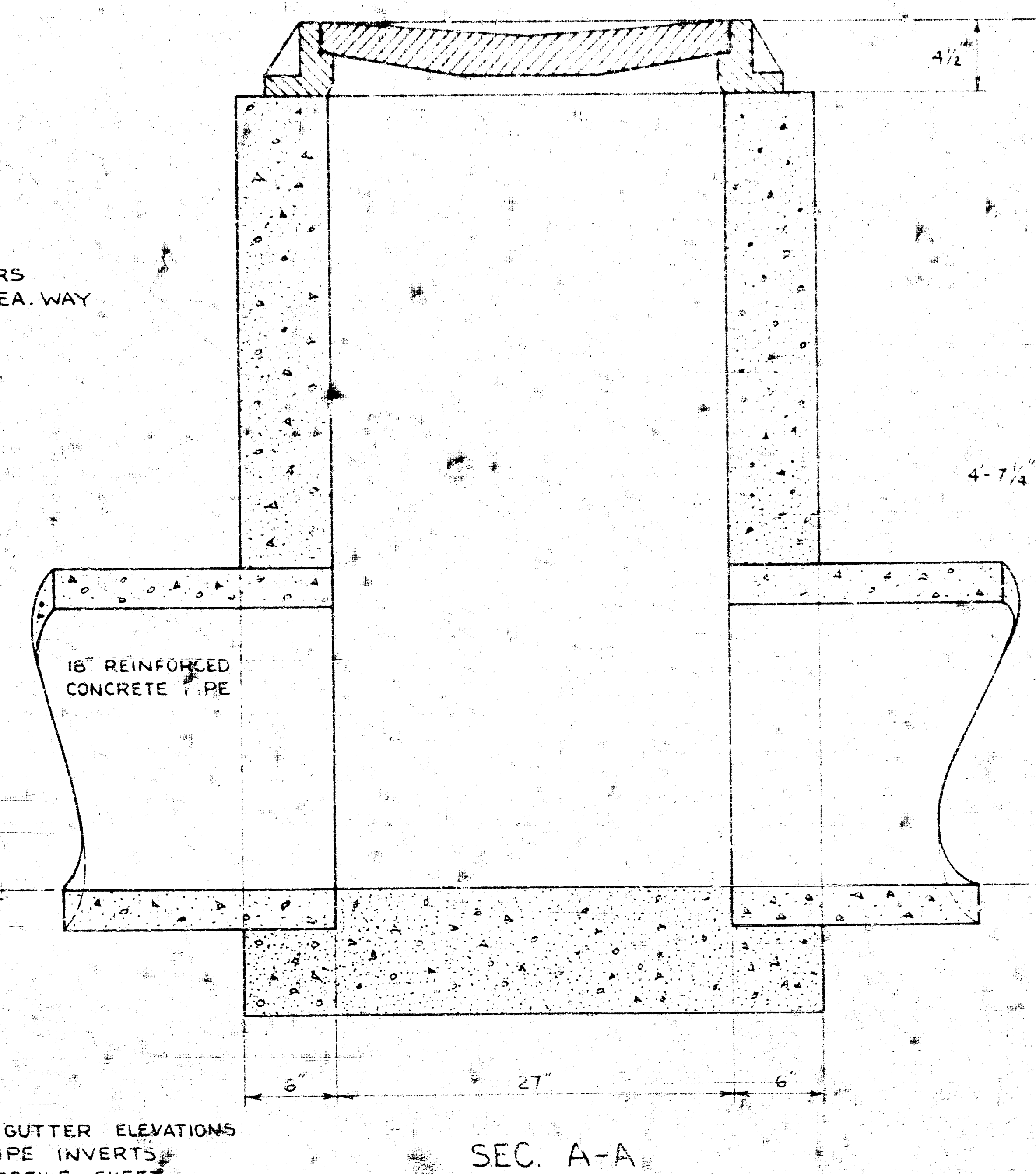
GUTTER INLET DETAIL TYPE - B SCALE 1/2" = 1'-0"
