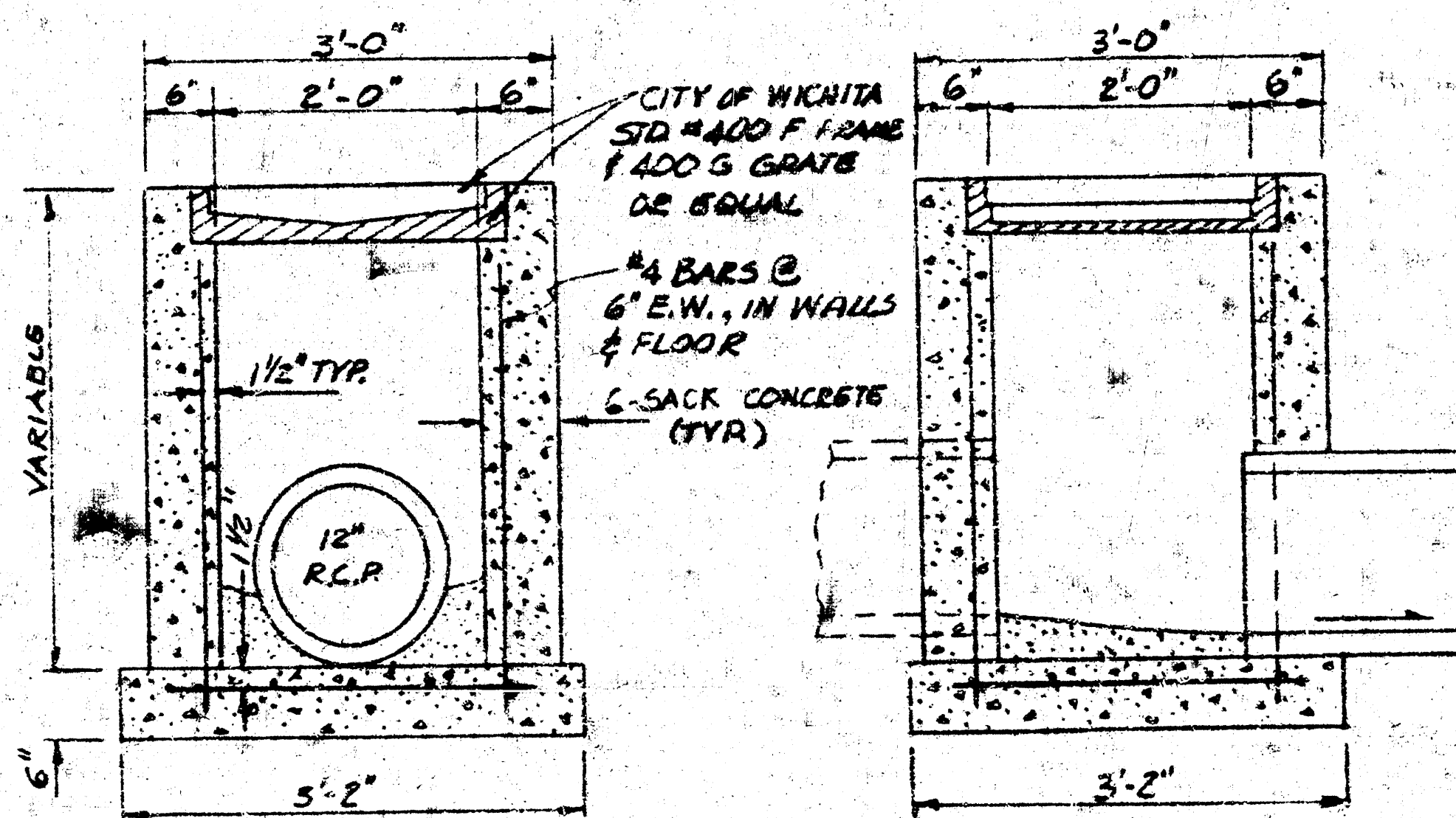
REINFORCED CONCRETE DROP INLET (ALTERNATE)
