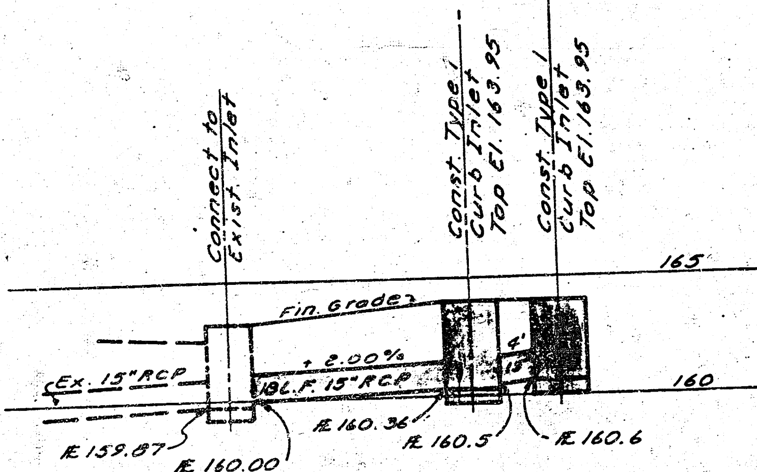
STORM SEWER PROFILE Scale: Hor. 1"=10' Ver. 1"=5'
