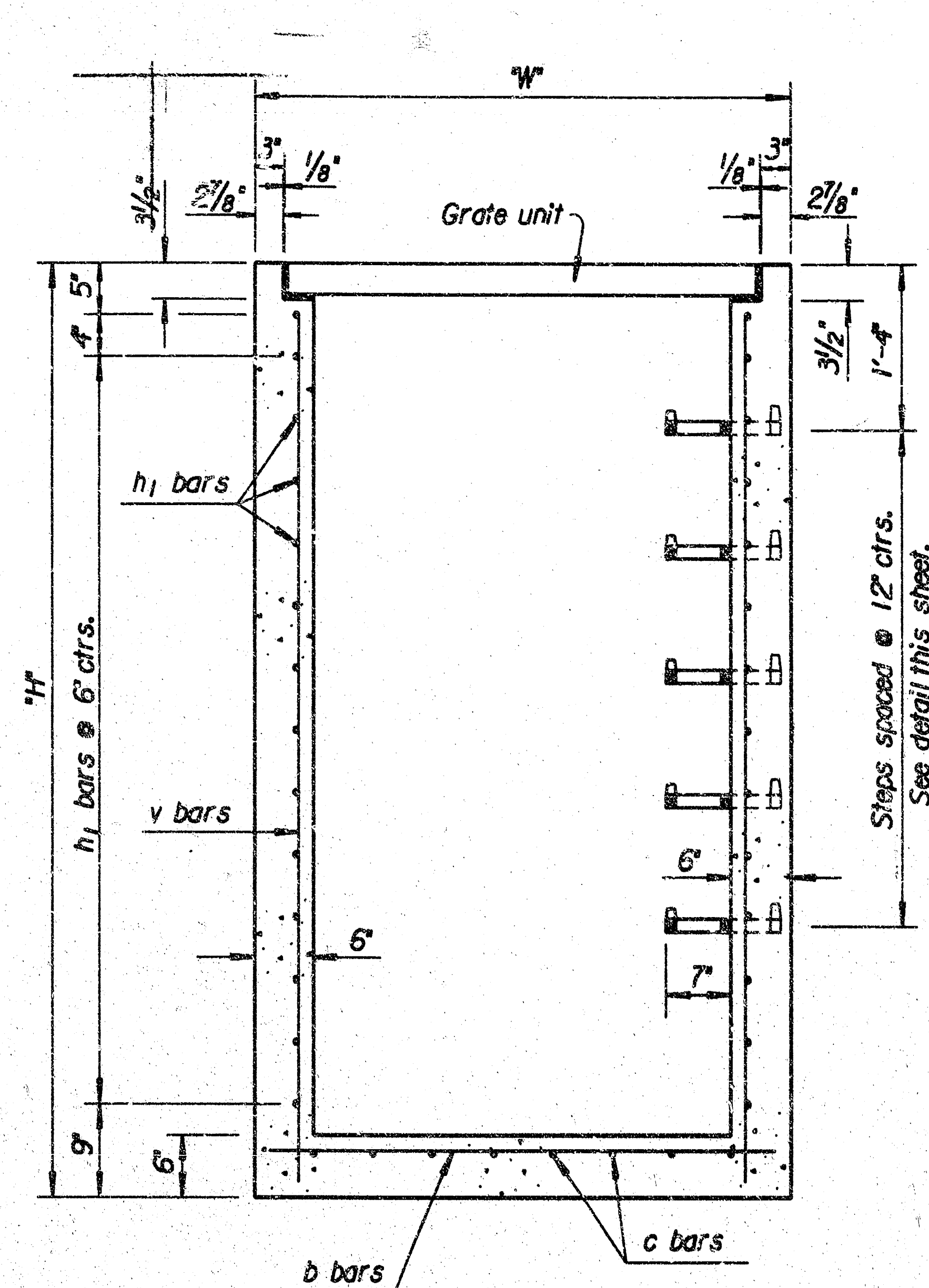
SECTION
