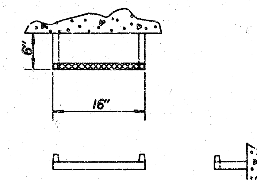
STEP DETAILS
