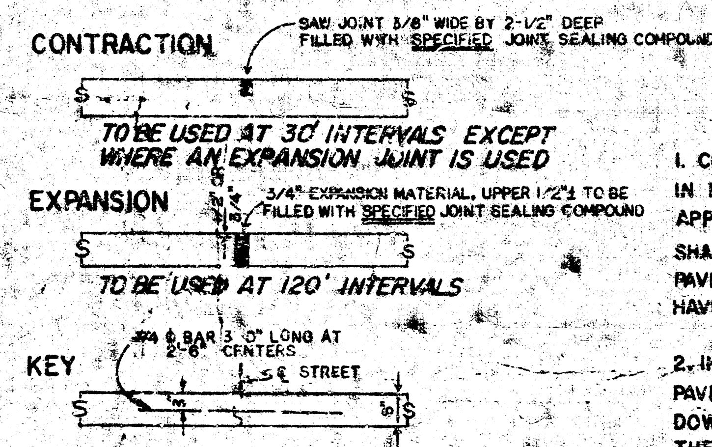
JOINT DETAILS
