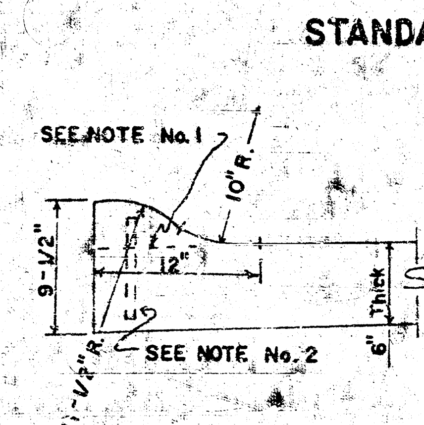
ROLL-TYPE
