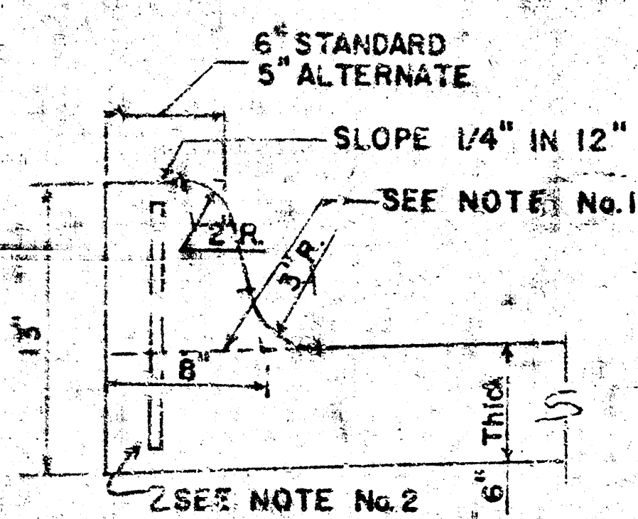
INTEGRAL CURB
