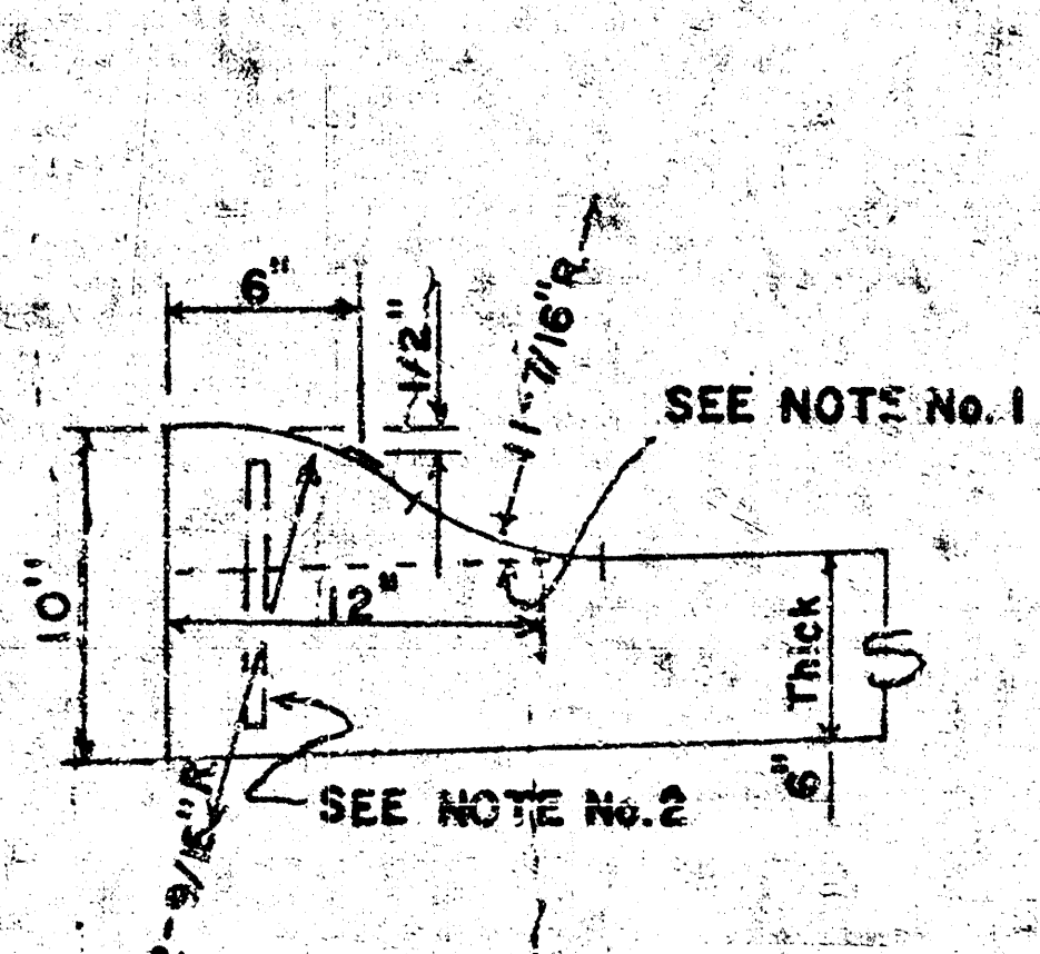
ALTERNATE ROLL-TYPE
